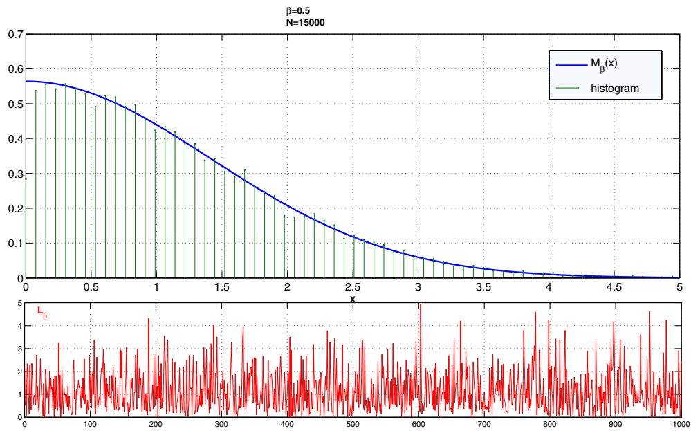
Figure 2. In the top panel, the histogram for the case \beta = 0.5 is calculated from a sample of N = 15000 outcomes, which are obtained simulating independent Gaussian random variables. The corresponding L_\beta is shown in the bottom.
