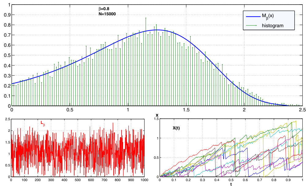
Figure 3. In the top panel, the histogram of L_\beta , which is calculated from a sample of N = 15000 outcomes, is obtained with an explicit random walk scheme and is compared with the exact PDF M_\beta(x), x \geq 0 , with \beta = 0.8 . In the bottom panels, the random variable L_\beta (left) and many trajectory examples (right) are shown.
