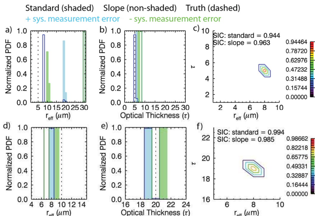
Figure 6. Marginal pdfs in effective radius ( r_{\text{eff}} , in \mu\text{m} ) and optical thickness and the joint posterior pdf for (a–c) true \tau , r_e = 5 , 5 \mu\text{m} and for (d–f) true \tau , r_e = 20 , 10 \mu\text{m} . Marginal pdf results are shown for standard (shaded histograms) and slope (non-shaded histograms) methods; the spread in the histograms results from \pm 3\% systematic measurement errors (‘+’ in blue; ‘-’ in green) and \pm 30\% uncertainty in water vapor. True values in \tau and r_e are indicated with vertical dashed lines. The joint posterior pdf (for the slope method) is shown with colored contours and the highest contour level is centered on the maximum likelihood solution. Shifts in the maximum likelihood solution from the true values represent retrieval biases. The normalized Shannon Information Content (SIC) in the joint posterior pdf for standard and slope methods is indicated on (c) and (f). Calculations shown are for \mu_0 = 0.866 .
