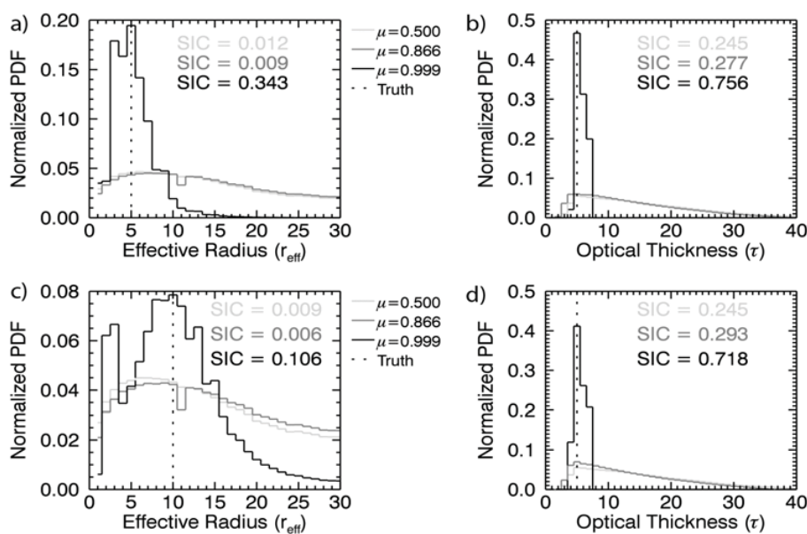
Figure 9. The dependency in the marginal pdfs in cloud optical thickness and droplet effective radius on solar zenith angle for true (a,b) \tau, r_e = 5, 5 \mu\text{m} , (c,d) \tau, r_e = 5, 10 \mu\text{m} , (e,f) \tau, r_e = 20, 5 \mu\text{m} , and (g,h) \tau, r_e = 20, 10 \mu\text{m} . True values in \tau and r_e are indicated with vertical dashed lines. Calculations were performed using the slope method for \mu_0 = 0.500 (light grey), \mu_0 = 0.866 (dark grey), and \mu_0 = 0.999 (black). The normalized Shannon information content in the marginal pdfs with changing \mu_0 is indicated on each plot using matching font colors.
