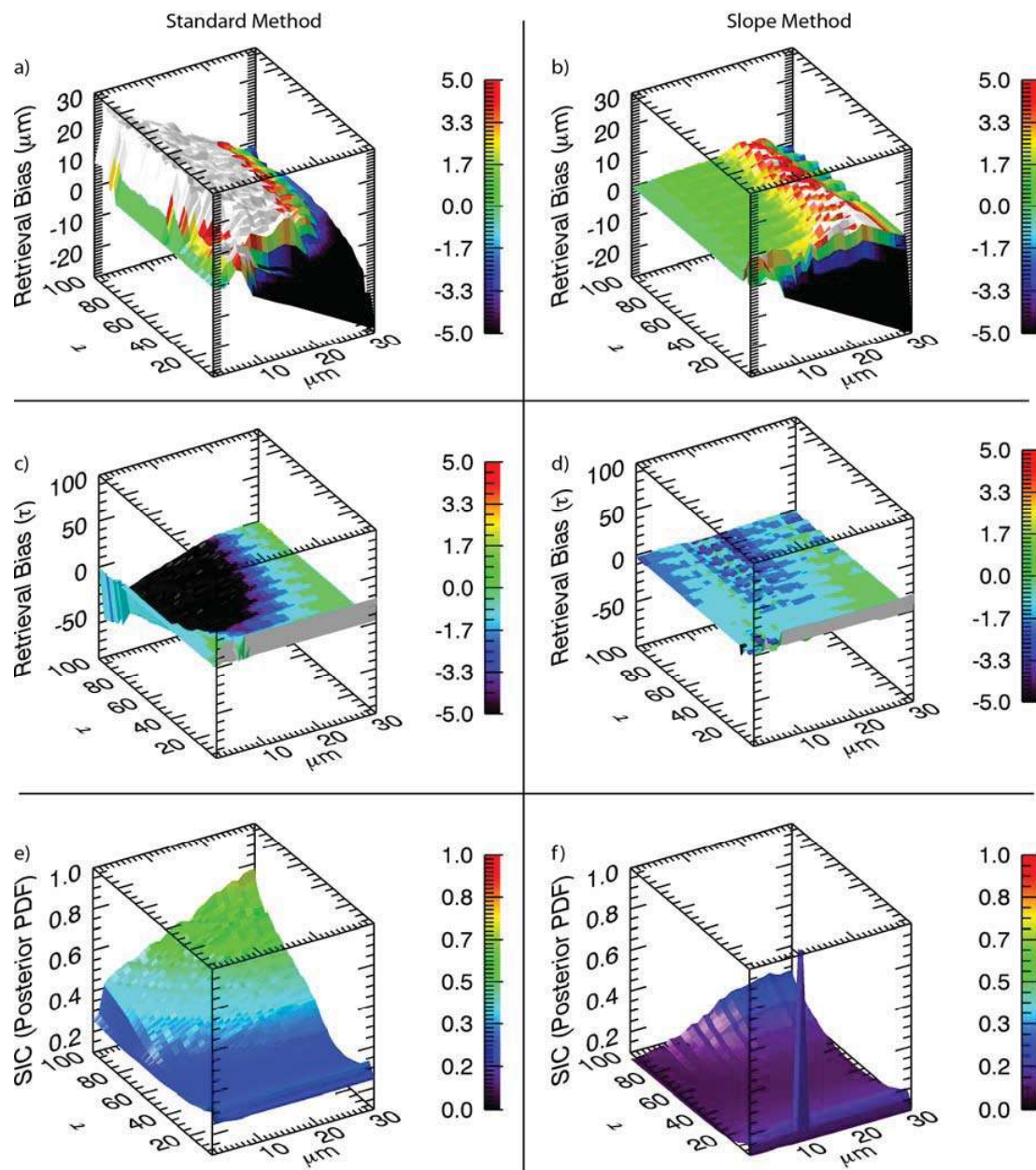
Figure 7. Surface plots of retrieval biases in effective radius and optical thickness (biases are defined as the difference between the maximum likelihood solution of the joint posterior pdf in \tau and r_e and the true values) and the normalized Shannon information content of the joint posterior pdf for the standard method (left column) and the slope method (right column,). Results (z-axis) are shown for a broad range in droplet effective radius (1–30 \mu\text{m} , x-axis) and cloud optical thickness (1–100, y-axis). Calculations shown are for \mu_0 = 0.866 , +3% systematic measurement error, and variable surface albedo from bare soil to purely vegetated surface types. Colored contours are used to ease interpretation of retrieval biases ( a–d ) within \pm 5 in optical thickness and \pm 5 \mu\text{m} in effective radius, where black denotes retrieval biases in excess of -5 and white denotes retrieval biases in excess of +5 . Green denotes near zero biases. In ( e,f ), the color scale of the normalized Shannon information content ranges from 0 to 1.
