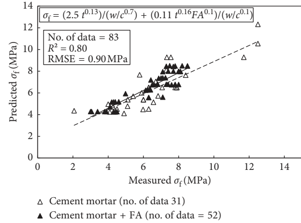
FIGURE 11: Relationship between measured and predicted flexural strengths for cement mortar with and without fly ash (FA).
