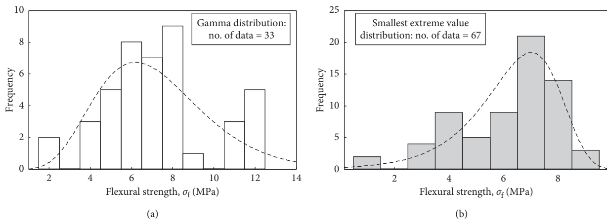
FIGURE 5: Statistical distribution of the flexural strength for (a) cement mortar and (b) cement mortar modified with fly ash (FA) up to 90 days of curing.
