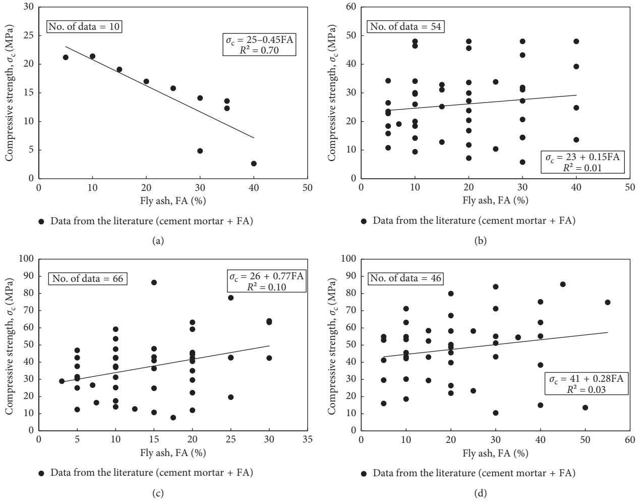
FIGURE 8: Variation between percentage of fly ash and compressive strength of cement mortar at different curing times: (a) 1 day; (b) 7 days; (c) 28 days; (d) 90 days.
