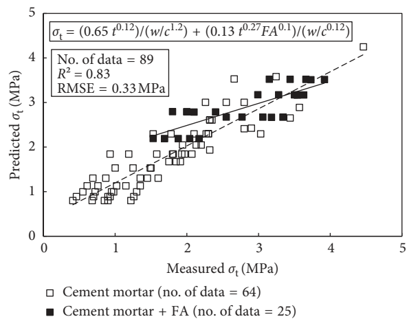
FIGURE 10: Relationship between measured and predicted split tensile strengths for cement mortar with and without fly ash (FA).
