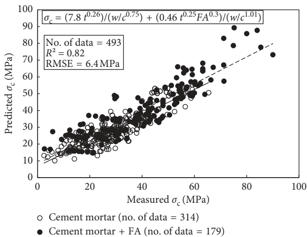
FIGURE 9: Relationship between measured and predicted compressive strengths for cement mortar modified with fly ash (FA).
