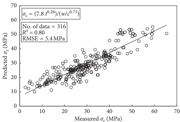
FIGURE 7: Relationship between measured and predicted compressive strengths for cement mortar.
