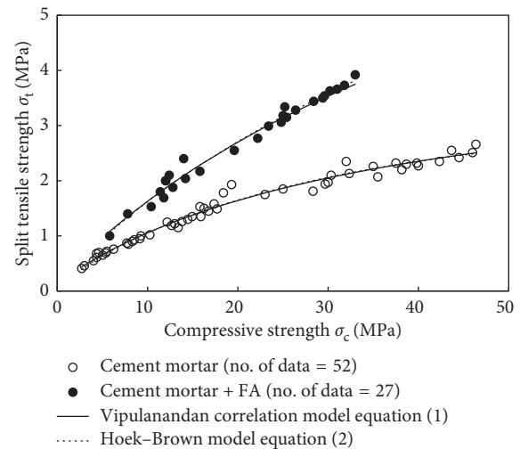
FIGURE 12: Variation of split tensile and compressive strengths of cement mortar with and without fly ash (FA).
