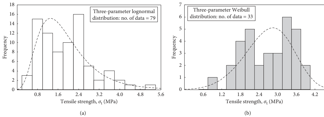
FIGURE 4: (a) Three-parameter lognormal distribution of the tensile strength for cement mortar and (b) 3-parameter Weibull distribution of the tensile strength for cement mortar modified with fly ash (FA) up to 90 days of curing.
