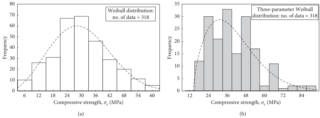
FIGURE 3: Statistical distribution of the compressive strength for (a) cement mortar and (b) cement mortar modified with fly ash (FA) up to 90 days of curing.
