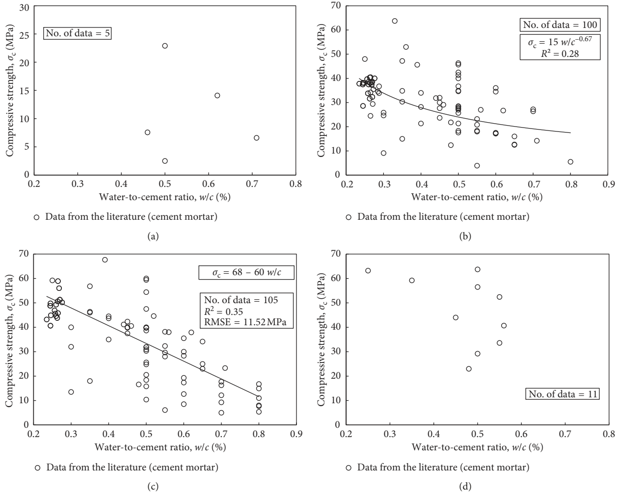
FIGURE 6: Variation between w/c and compressive strength of cement mortar at different curing times: (a) 1 day; (b) 7 days; (c) 28 days; (d) 90 days.
