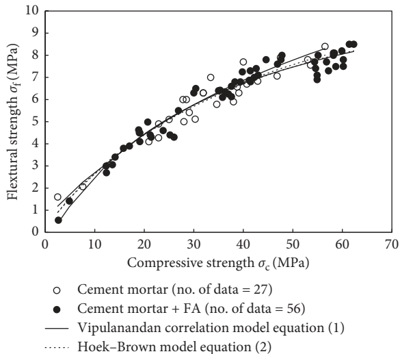
FIGURE 13: Variation of flexural and compressive strengths of cement mortar with and without fly ash (FA).
