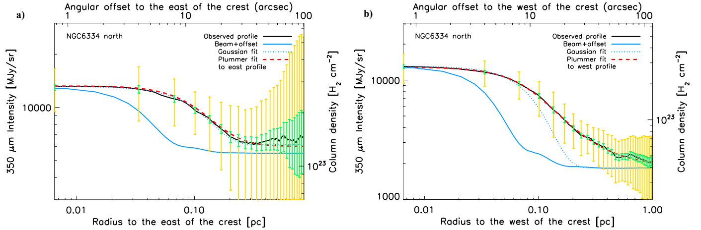
Fig. A.1. a) Median radial intensity profile of the northern part of the NGC 6334 filament (black solid curve) measured in the combined ArTéMiS + SPIRE 350 μm image (Fig. 1b) perpendicular to, and on the eastern side of, the filament crest shown as a white curve in Fig. 2a. The yellow and green error bars are as in Fig. 3a. The blue solid curve shows the effective beam profile of the ArTéMiS 350 μm data as measured on Mars, overlaid on a constant level corresponding to the typical background intensity level observed at large radii. The blue dotted curve shows the best-fit Gaussian (+ constant offset) model to the inner part of the observed profile. The red dashed curve shows the best-fit Plummer model convolved with the beam (cf. Sect. 3 and Eq. (2)). b) Same as in a) but for the median radial intensity profile of the northern part of the filament measured on the western side of the filament crest shown as a white curve in Fig. 2a.
