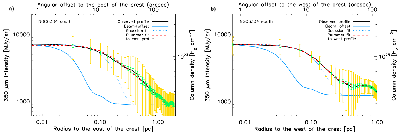
Fig. A.2. a) Median radial intensity profile of the southern part of the NGC 6334 filament (black solid curve) measured in the combined ArTéMiS + SPIRE 350 μm image (Fig. 1b) perpendicular to, and on the eastern side of, the filament crest shown as a magenta curve in Fig. 2a. The yellow and green error bars are as in Fig. 3a. The blue solid curve shows the effective beam profile of the ArTéMiS 350 μm data as measured on Mars, overlaid on a constant level corresponding to the typical background intensity level observed at large radii. The blue dotted curve shows the best-fit Gaussian (+ constant offset) model to the inner part of the observed profile. The red dashed curve shows the best-fit Plummer model convolved with the beam (cf. Sect. 3 and Eq. (2)). b) Same as in a) but for the median radial intensity profile of the southern part of the filament measured on the western side of the filament crest shown as a magenta curve in Fig. 2a.
