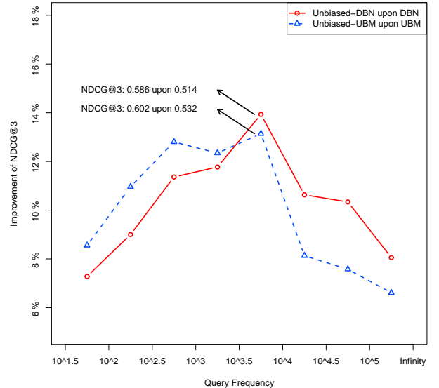
Figure 5: The relative NDCG improvement over query frequencies
