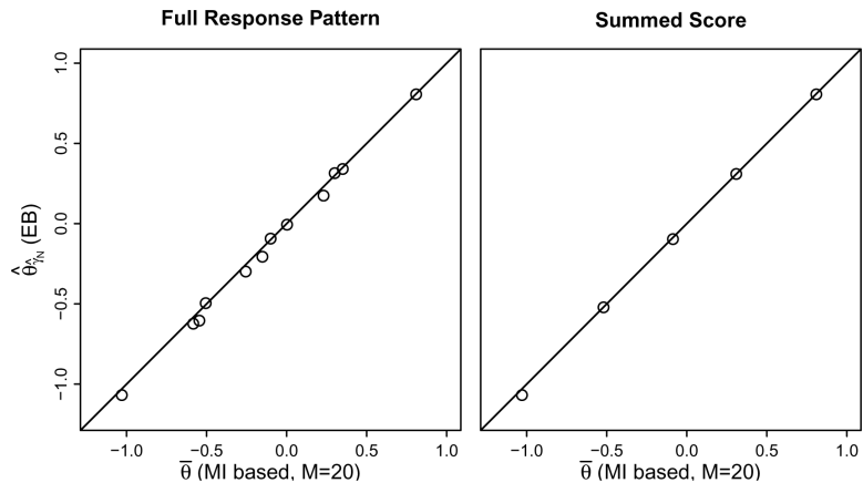
Figure 2. Traditional and MI based EAP estimates.
