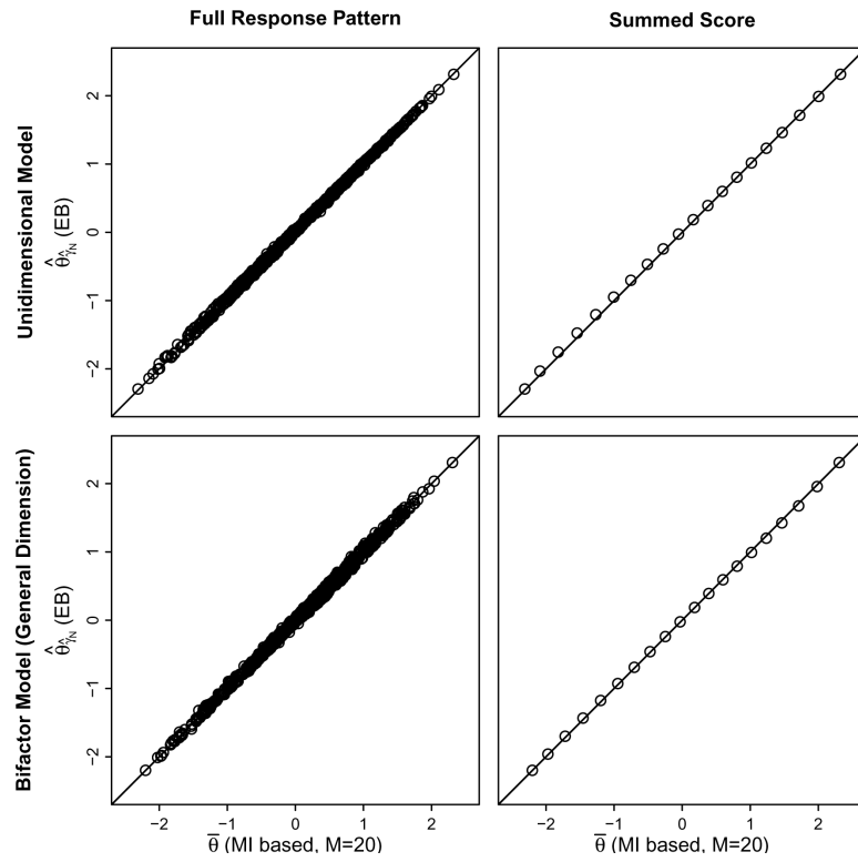
Figure 6. Estimated IRT Scale Scores for PISA Math Booklet 8.
