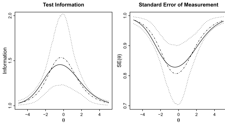
Figure 5. Confidence envelopes for test information and the conditional SEM. Solid curves show test information and the conditional SEM based on the MML item parameter estimates. The dotted curves represent the 95% confidence limits. The expected information and conditional SEM curves are shown as dashed lines. The confidence limits and expected functions are based on M = 1000 imputations.
