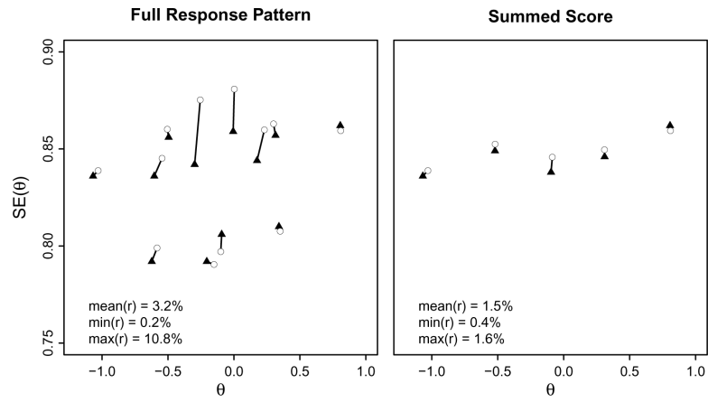
Figure 3. MI based scale score and SEM corrections. Traditional estimates are represented by the closed triangles. MI based estimates are shown as open circles.
