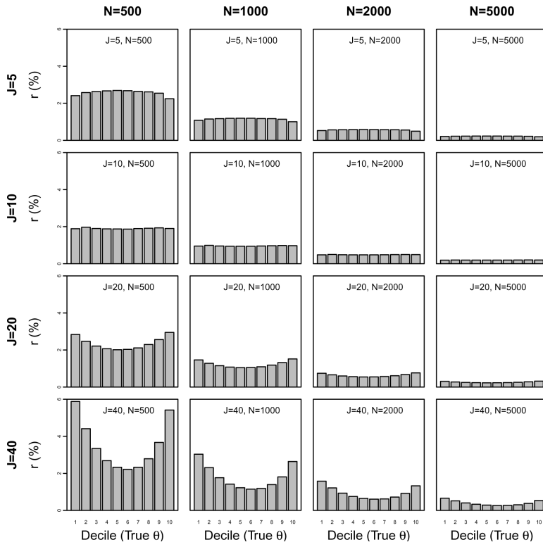
Figure 9. Mean relative increase in variance (by deciles) under various simulated test lengths and calibration sample sizes for the logistic graded response model with 5 categories.
