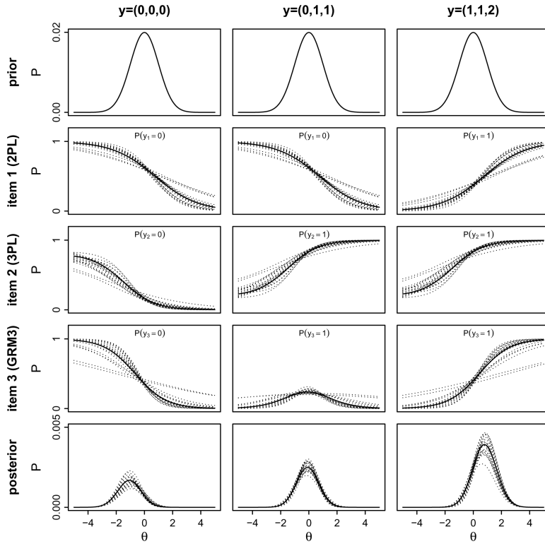
Figure 1. Item trace lines and posterior distributions for three response patterns. Solid lines represent the tracelines and posteriors based on the MML parameter estimates; those based on M=20 randomly imputed parameter sets appear as dotted lines.
