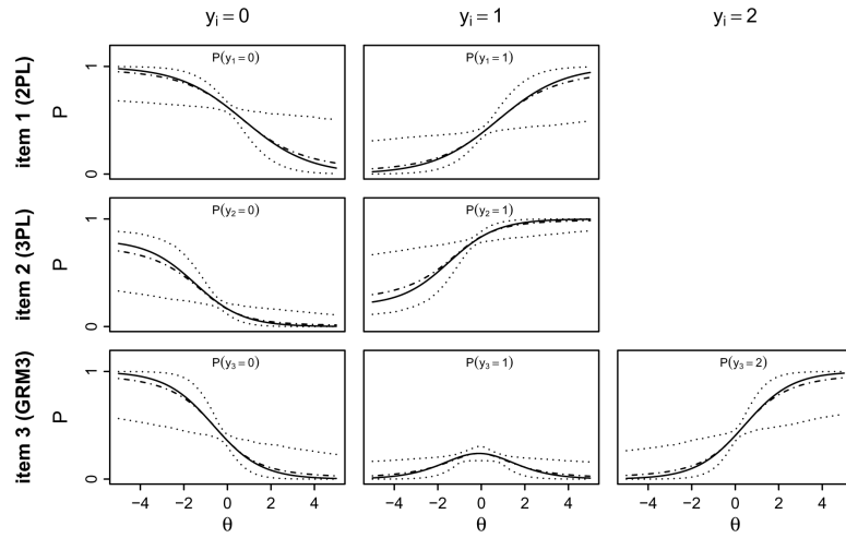
Figure 4. Confidence envelopes for item tracelines. The solid curves represent the item characteristic curves based on the MML item parameter estimates. The dotted curves represent the 95% confidence limits. The dashed curves show the expected response functions. The confidence limits and expected functions are generated based on M = 1000 imputations
