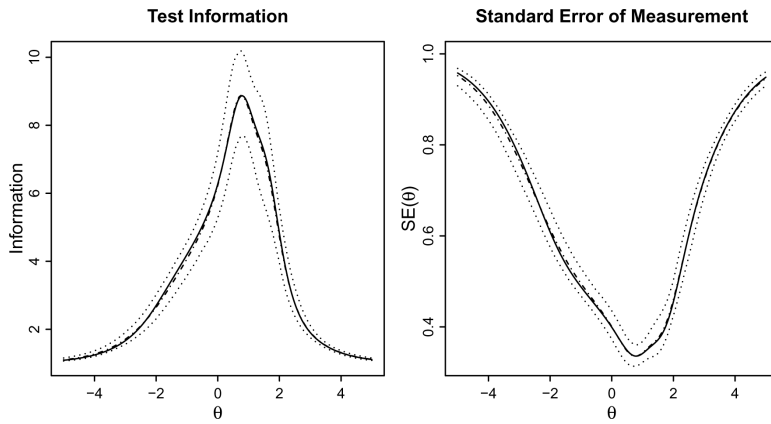
Figure 8. Confidence envelopes for test information and the conditional SEM for PISA Math Booklet 8. The solid curves show test information and the conditional SEM based on the MML item parameter estimates. The dotted curves represent the 95% confidence limits. The expected information and conditional SEM curves are shown as dashed lines. The confidence limits and expected functions are based on M = 1000 imputations.
