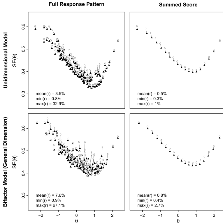
Figure 7. Traditional and MI based response pattern and summed score SEM estimates plotted against EAPs for PISA Math Booklet 8. For clarity, values for 200 randomly selected individuals in the scoring sample are plotted; the mean, minimum, and maximum values of r are based on the full scoring sample of 1000 individuals. Traditional estimates and SEMs based on the MML item parameters are shown as triangles. MI based results are shown as circles.
