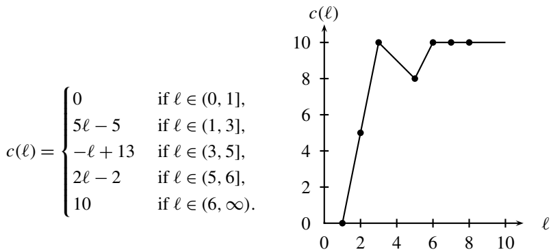
Fig. 1 A non-linear cost function c_f that gives rise to an exact potential in all weighted congestion games with demands d_1 = 1, d_2 = 3 and d_3 = 5
