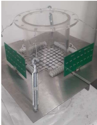
Fig. 5 Picture of the wire-mesh electrostatic sensor
