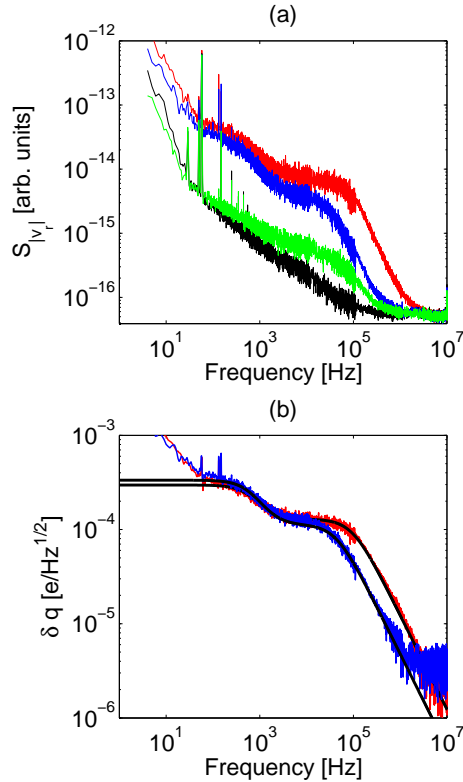
FIG. 3: (color online) (a) Power spectral density (PSD) of the reflected voltage measured in the points A (black curve); B (blue curve); C (green curve); D (red curve). (b) Normalized noise in the points B (blue curve); D (red curve). The black continuous lines are a fits to the measured PSD with a sum of two Lorentzian functions.
