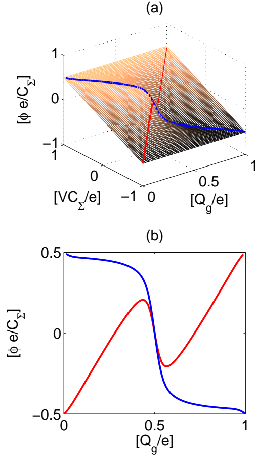
FIG. 6: (color online) (a) The SET island potential \phi calculated from the orthodox theory, as a function of bias voltage and gate charge. (b) Line cuts along the two diagonals in (a), where the measurements have been performed. As can be seen the potential is asymmetric with respect to the SET degeneracy point. If the grain SEB is biased away from its degeneracy point the frequency of the tunneling on and off the grain should be proportional to the island potential. The resulting fit is shown in figure 7.
