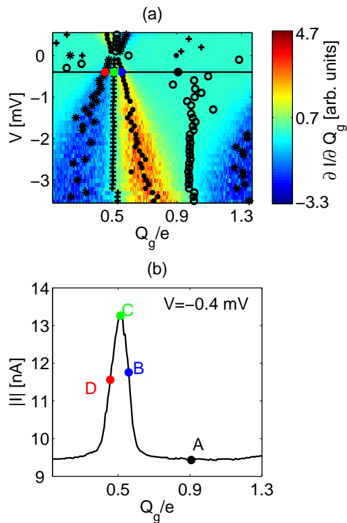
FIG. 2: (color online) (a) The SET stability diagram ( \partial I / \partial Q_g ) measured at a temperature of 25 mK. Horizontal black line corresponds to the bias voltage, where transfer function I(Q_g) (see panel (b)) was obtained. The points A / (( \circ ) for negative and ( + ) for positive bias) where I = 0 inside the Coulomb blockade region. The points B and D ( */\bullet ) correspond to maximum positive/negative gain, \partial I / \partial Q_g that is where \partial^2 I / \partial Q_g^2 = 0 . The measurement points C , close to the current maximum current, correspond to \partial I / \partial Q_g = 0 , marked with ( + ) at negative bias and with ( \circ ) at positive bias. (b) SET transfer function I(Q_g) measured for the bias voltage V = -0.4 mV. In the stability diagram this measurements is shown as a black line.
