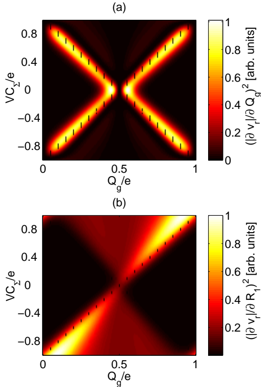
FIG. 1: (color online) Calculated derivatives from equation (1) as a function of bias voltage V , and gate charge Q_g = C_g V_g . The derivative of the reflected voltage from the rf-SET with respect to (a) the charge fluctuations (\partial|v_r|/\partial Q_g)^2 ; (b) the resistance fluctuations in the 1st junction (\partial|v_r|/\partial R_1)^2 . Sensitivity to the resistance fluctuations in the second junction has a mirror symmetry, along SET open state ( Q_g = 0.5e ), with the sensitivity to the resistance fluctuations in the first barrier.
