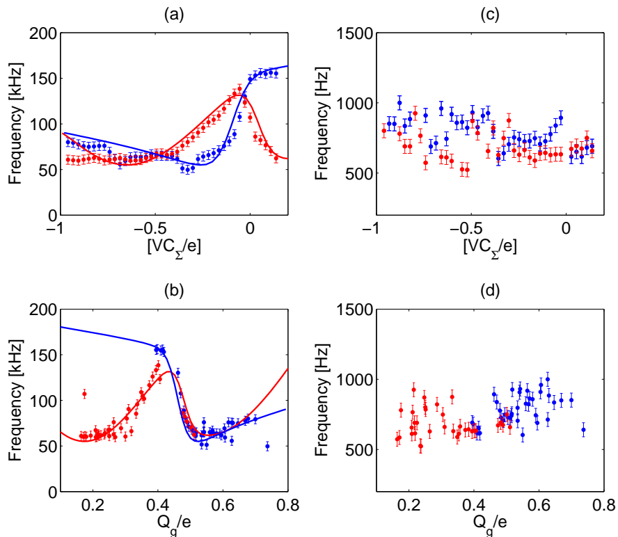
FIG. 4: (color online) (a) The bias dependence of the cut-off frequency for the high frequency Lorentzian. (b) The gate dependence of the cut-off frequency for the high frequency Lorentzian. (c) The bias dependence of the cut-off frequency for the low frequency Lorentzian. (d) The gate dependence of the cut-off frequency for the low frequency Lorentzian. Blue points correspond to the negative slope \partial I/\partial Q_g > 0 (see fig. 2). Red points correspond to the positive slope \partial I/\partial Q_g < 0 (see fig. 2). The error bars are extracted from the fits to the Lorentzians. The continuous lines (blue, red) show the bias and gate dependencies for the Lorentzian cut-off frequency calculated in the described model.
