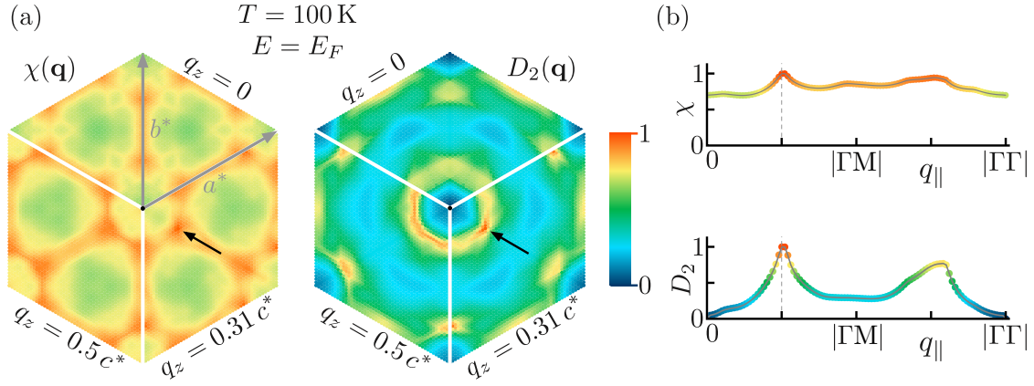
Figure 2: (a) The Lindhard function \chi(\mathbf{q}) (left) and the structured susceptibility D_2(\mathbf{q}) (right) at T = 100 K as a function of in-plane q_{\parallel} (with q_{\parallel} = 0 indicated by the black dot), at various values of q_z . Both graphs are normalised to their respective maxima, which lie around \mathbf{q} = (0, 0.25, 0.31) rlu and symmetry-related positions (black arrows). (b) Line cuts of the Lindhard function and structured susceptibility at q_z = 0.31c^* , varying q_{\parallel} along a line through the black arrows in (a).
