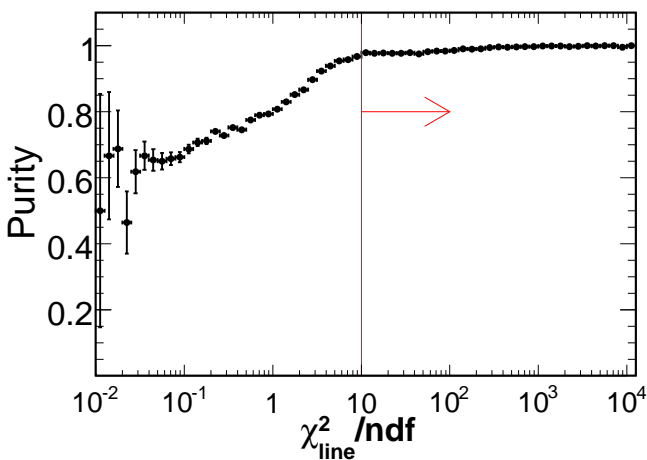
FIG. 9: Purity of the charge sign determination for neutrino-induced muons as a function of \chi_{\text{line}}^2/ndf . Events with \chi_{\text{line}}^2/ndf > 10 have well-determined charge sign and momentum.
