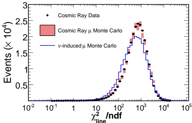
FIG. 8: Comparison of the \chi_{\text{line}}^2/ndf distributions for stopping muons in the cosmic ray data (points), in the cosmic ray Monte Carlo simulation (boxes), and in the neutrino-induced Monte Carlo simulation (line). The vertical extent of the boxes representing the cosmic ray Monte Carlo simulation indicate the statistical uncertainty for the points.
