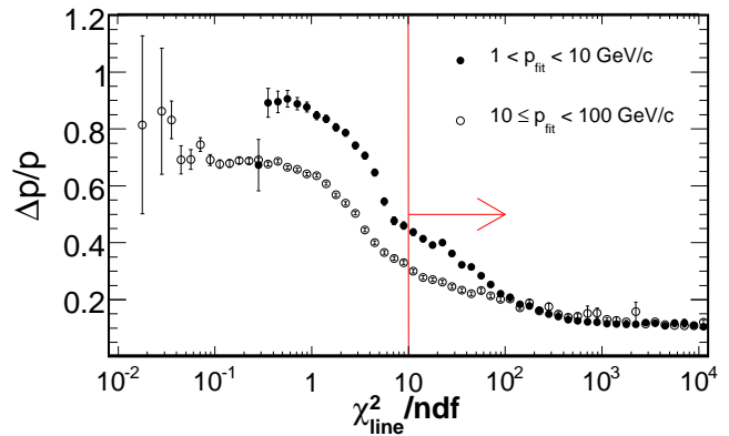
FIG. 10: Momentum resolution for Monte Carlo neutrino-induced muons as a function of \chi_{\text{line}}^2/ndf . The line at \chi_{\text{line}}^2/ndf = 10 shows the cut used in the analyses.
