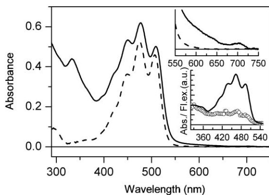
Fig. 2 Absorption spectra of C-C 60 dyad (solid line) and of the model carotenoid (dashed line) in toluene. The upper inset shows the expanded absorption spectra. The lower inset shows the absorption (solid line) and fluorescence excitation (circles) spectra in hexane.
