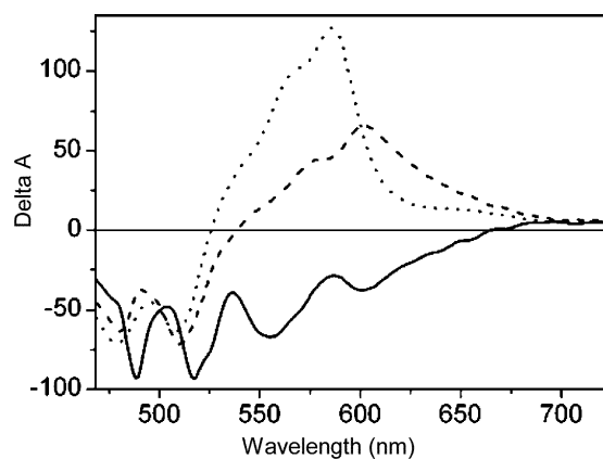
Fig. 3 Evolution associated difference spectra (EADS) that follow from the global analysis of the time-resolved experiments on the model carotenoid in toluene with excitation at 475 nm. Lifetimes: 100 fs (solid line, fixed), 300 fs (dashed line) and 7.6 ps (dotted line).
