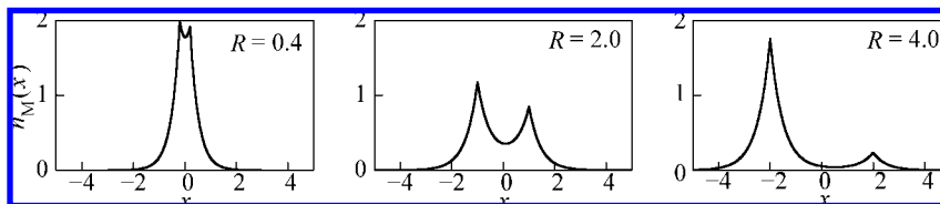
Figure 1. Molecular density for three different internuclear separations: R = 0.4 (left), R = 2.0 (center), and R = 4.0 (right). In this plot, Z_A = 1.02 , and Z_B = 0.98 .
