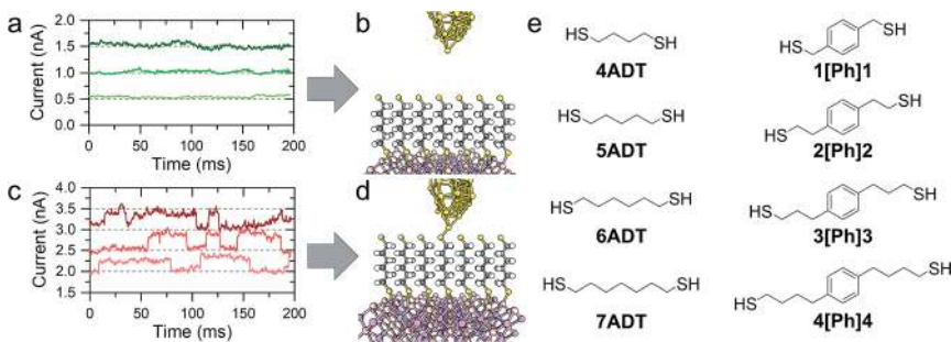
Fig. 1 (a) Tunneling readout at low setpoint bias, where the tip is not in contact with the monolayer, as depicted in (b). (c) Tunneling readout at higher setpoint bias, where the sudden jumps are related to the formation of Au-S bonds between the tip and the monolayer thiolated termini (d). (e) Structure of molecular wires employed in this study.
