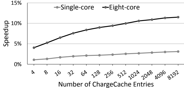
Figure 10: Speedup versus ChargeCache capacity.
