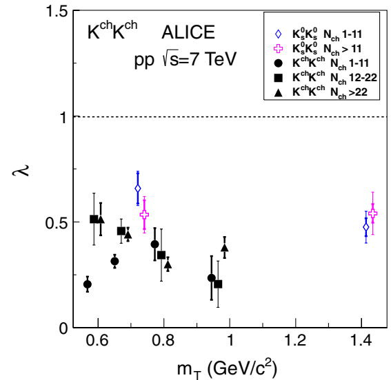
FIG. 3 (color online). \lambda parameters of K^{\text{ch}}K^{\text{ch}} versus m_T extracted by fitting correlation functions shown in Fig. 2 to Eq. (1) and the baseline to Eq. (2). For comparison, the K_s^0 K_s^0 [10] \lambda parameters measured by ALICE in 7 TeV pp collisions are also shown. Statistical (darker lines) and total errors are shown. The points corresponding to the second and third multiplicity bins are offset by 0.03 GeV/ c^2 for clarity.
