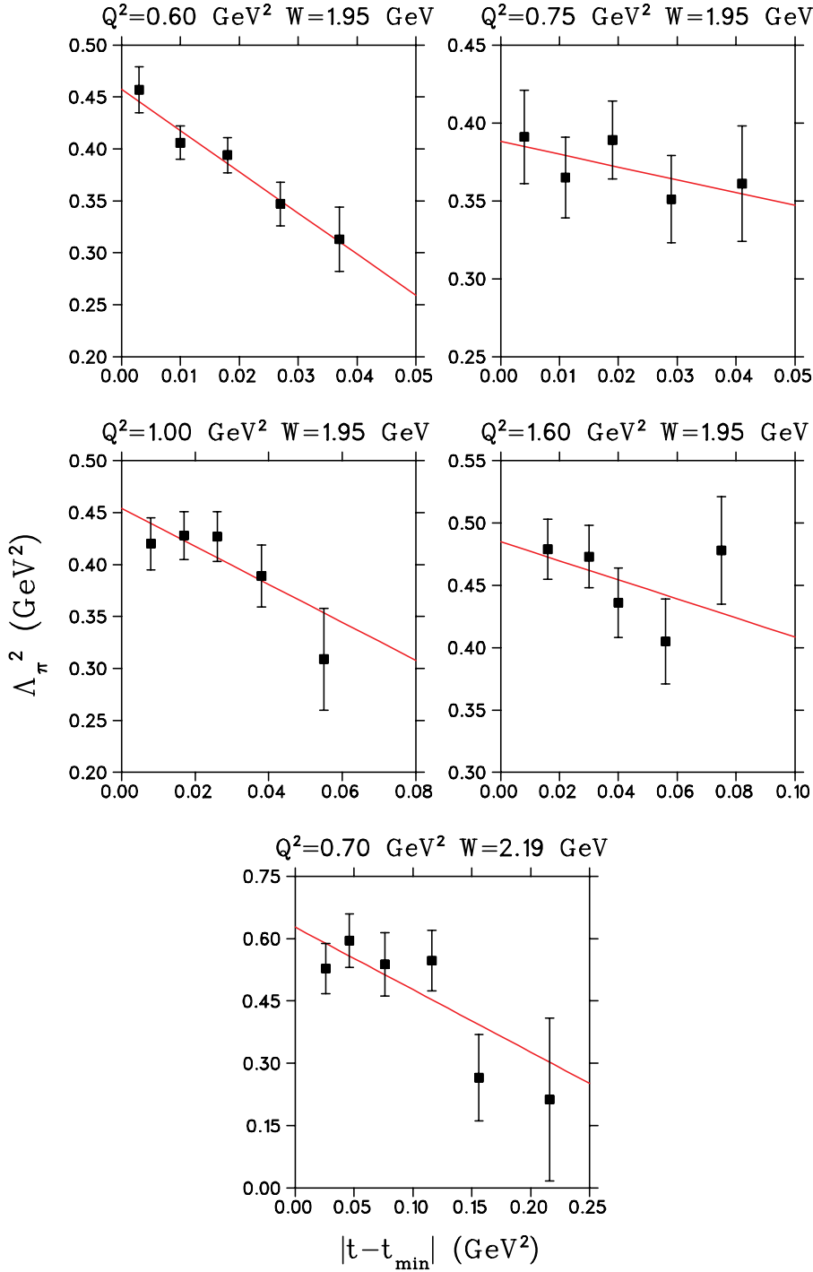
FIG. 5. (Color online) Values of \Lambda_\pi^2 determined from the fit of the VGL model to each t bin and linear fit to same. The error bars reflect the statistical and t -uncorrelated systematic uncertainties. The additional overall systematic uncertainties, which were applied after the fit, are not shown.
