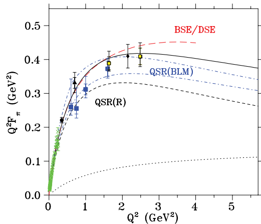
FIG. 9. (Color online) The F_\pi data of Fig. 6 are compared with the QCD sum rules calculations of Refs. [6,69] and the Bethe-Salpeter equation model utilizing dressed quark propagators via the Dyson-Schwinger equation of Ref. [78] (long dashed). For the calculation of Ref. [69], three curves are shown: (dotted) F_\pi^{\text{hard}} , (short-dashed) F_\pi^{\text{soft}} , and (solid) the sum F_\pi^{\text{soft}} + F_\pi^{\text{hard}} . For the calculation of Ref. [6], two dot-dashed curves are shown: (lower) s_0 = \frac{4\pi^2 f_\pi^2}{1+\alpha_s(Q^2)/\pi} , (upper) s_0 = 0.65 \text{ GeV}^2 .
