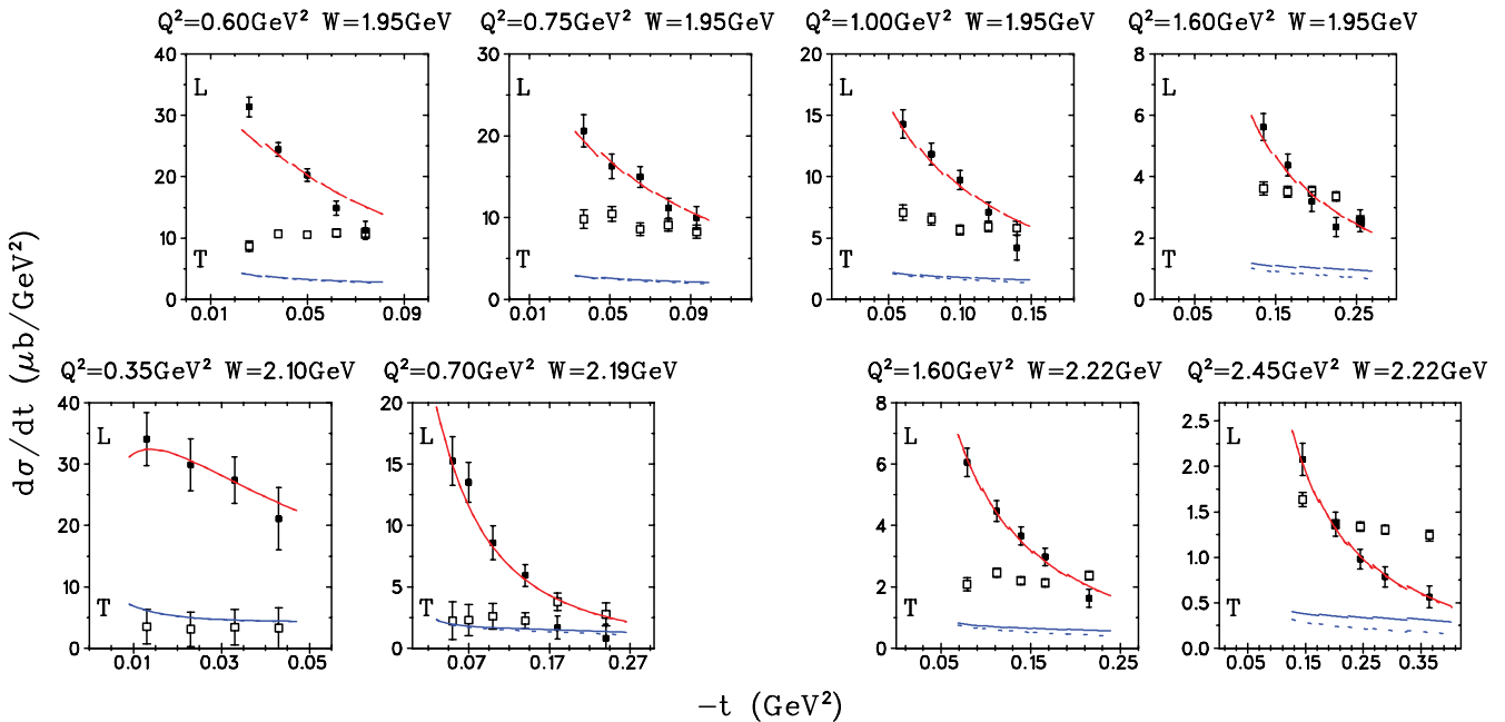
FIG. 2. (Color online) Separated \pi^+ electroproduction cross sections \sigma_L (solid) and \sigma_T (open) from JLab and DESY in comparison to the predictions of the VGL Regge model [23]. The error bars of the JLab data represent the combination of statistical and t uncorrelated systematic uncertainties. In addition, there is an overall systematic uncertainty of about 6%, mainly from the t -correlated, \epsilon -uncorrelated systematic uncertainty. The VGL Regge model calculations for Q^2 = 0.60 – 1.60 \text{ GeV}^2 , W = 1.95 \text{ GeV} use \Lambda_\pi^2 = 0.394, 0.372, 0.411 , and 0.455 \text{ GeV}^2 , and those for Q^2 = 0.35 – 2.45 \text{ GeV}^2 , W \sim 2.1 \text{ GeV} use \Lambda_\pi^2 = 0.601, 0.519, 0.513 , and 0.491 \text{ GeV}^2 . The solid(dashed) curves indicate the \Lambda_\rho^2 = 1.500(0.600) \text{ GeV}^2 value used.
