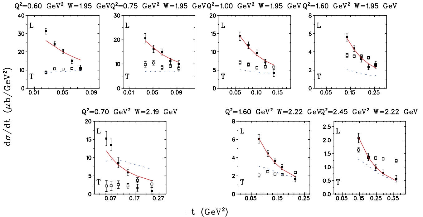
FIG. 3. (Color online) Separated \pi^+ electroproduction cross sections \sigma_L (solid) and \sigma_T (open) from this work and DESY [14] in comparison to the FGLO effective Lagrangian model [39]. The data error bars and systematic uncertainties are as in Fig. 2. The solid (dashed) curves denote model calculations for \sigma_L ( \sigma_T ) with \Lambda_\pi^2 = 0.405, 0.414, 0.503, 0.654, 0.386, 0.608, and 0.636 \text{GeV}^2 (from upper left to lower right). The calculations were performed at the same \bar{W} and \bar{Q}^2 as the data, with straight lines connecting the calculated values.
