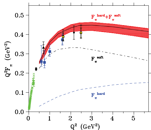
FIG. 7. (Color online) The F_\pi data of Fig. 6 are compared with a hard LO+NLO contribution by Bakulev et al. [47] based on an analysis of the pion-photon transition form-factor data from CLEO [48] and CELLO [49]. A soft component, estimated from a local quark-hadron duality model, is added to bring the calculation into agreement with the experimental data. The band around the sum reflects nonperturbative uncertainties from nonlocal QCD sum rules and renormalization scheme and scale ambiguities at the NLO level.
