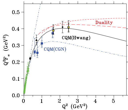
FIG. 10. (Color online) The F_\pi data of Fig. 6 are compared with the local quark-hadron duality analysis of W. Melnitchouk [84,85], and the constituent quark model calculations of Refs. [92,93]. For the duality calculation, two curves are shown: (short-dashed) leading-order analysis of Ref. [84], (long-dashed) next-to-leading order analysis of Ref. [85]. For the quark model calculations by Cardarelli et al. [92], two curves are shown: (upper dot-dashed) pointlike quarks and (lower dot-dashed) quarks with a monopole form factor.
