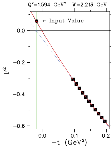
FIG. 1. (Color online) Linear (dotted), quadratic (dashed), and cubic (solid line) extrapolations of F_\pi^2 to the pole as computed from Eq. (6). The boxes are a VGL Regge model calculation for \sigma_L at fixed W = 2.213 GeV and Q^2 = 1.594 GeV 2 , calculated with F_\pi = 0.244 . The lower limit of the box range is the kinematic end point of these Q^2 , W values, whereas the upper limit is given by the t range of our experiment. The input F_\pi value in the model is indicated by the bullet placed at the pion pole.
