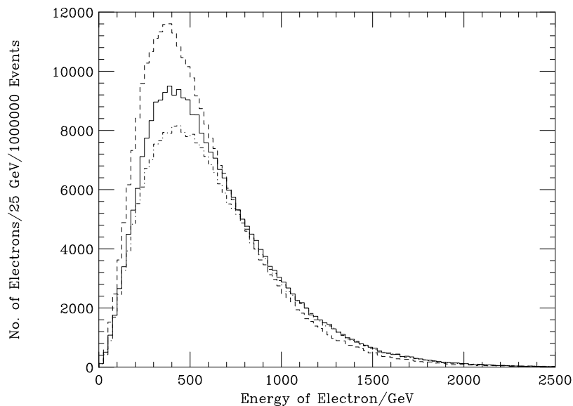
Figure 2: Parton-level energy spectra of electrons and positrons. As figure 1 but for electron and positron spectra.
