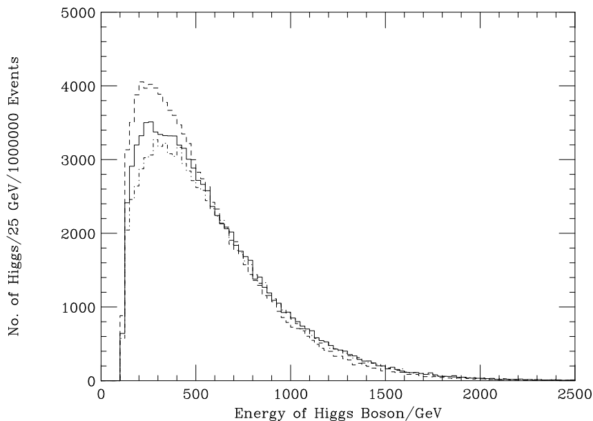
Figure 1: Parton-level energy spectra of Higgs bosons, m_H = 115 GeV. Solid: predicted energy spectrum of Higgs bosons from decay of black holes with initial masses 5.0 – 5.5 TeV. Dashed: neglecting time variation of temperature. Dot-dashed: neglecting grey-body factors.
