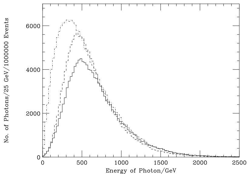
Figure 3: Parton-level energy spectra of photons. As figure 1 but for photon spectra.
