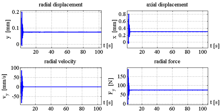
Fig. 14. Time histories of tool displacements and cutting forces in case with control, k_1 = 4
