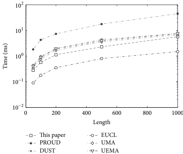
FIGURE 16: Average CPU time per query for Normal error distribution with varying length.
