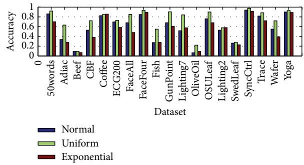
FIGURE 11: Accuracy of 19 datasets on three error distributions with accuracy of 1.4 and 2.0 mixed deviation.
