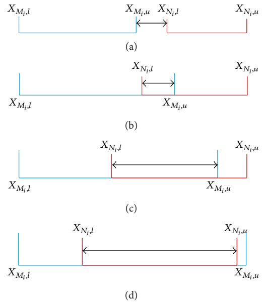
FIGURE 6: The illustration of similarity degrees.
