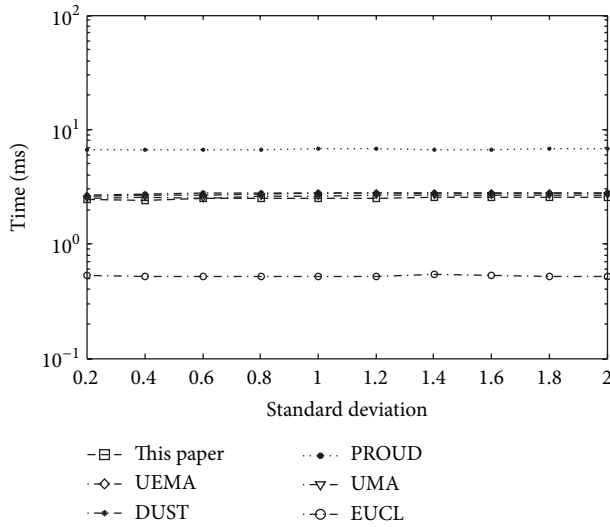
FIGURE 15: Average CPU time per query for Normal error distribution with varying deviation.
