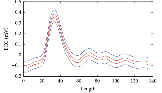
FIGURE 5: Illustration of smoothed Chebyshev uncertain time series after wavelet dimensionality reduction.
