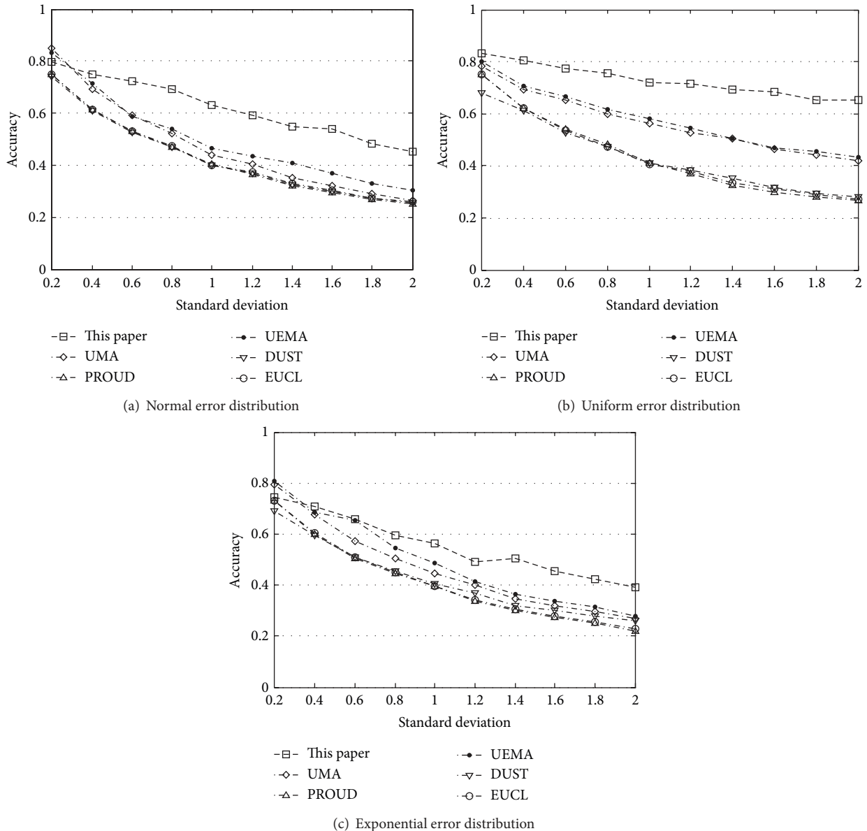
FIGURE 14: Comparison of accuracy with existing methods.
