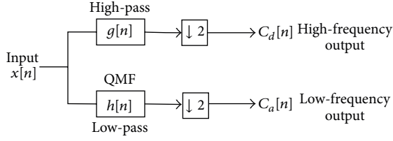
FIGURE 4: QMF wavelet transform for dimensionality reduction.
