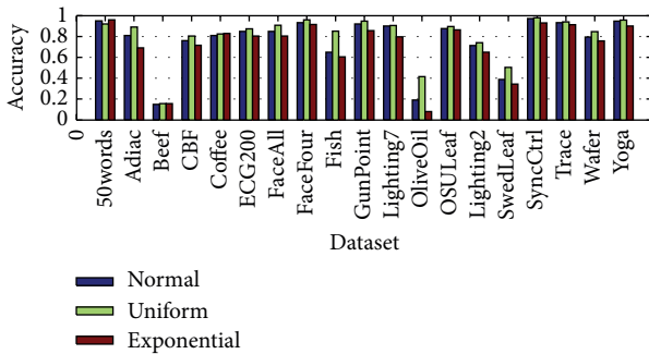
FIGURE 10: Accuracy of 19 datasets on three error distributions with accuracy of 0.4 and 1.0 mixed deviation.
