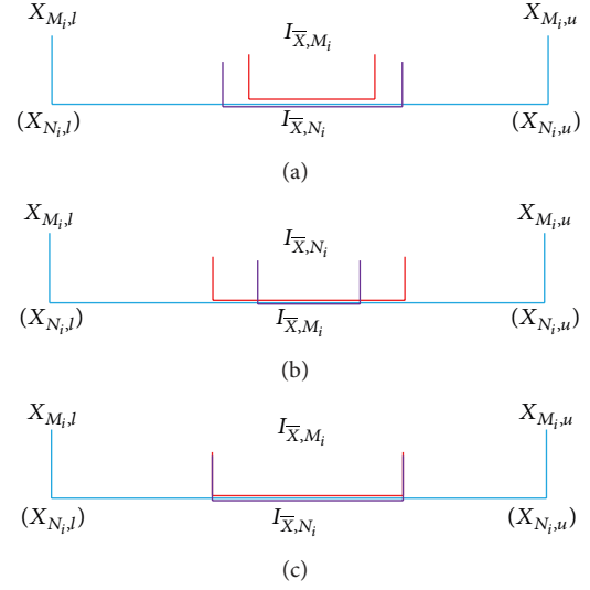
FIGURE 7: The situations of entire overlapping.
