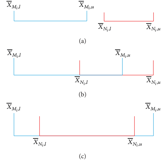
FIGURE 8: The illustration of overlap between \bar{X} intervals.
