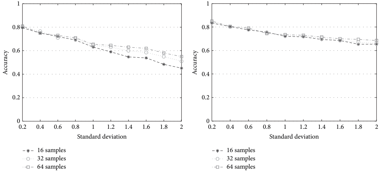
(a) Accuracy of 16, 32, and 64 sample observations with Normal error (b) Accuracy of 16, 32, and 64 sample observations with Uniform error
