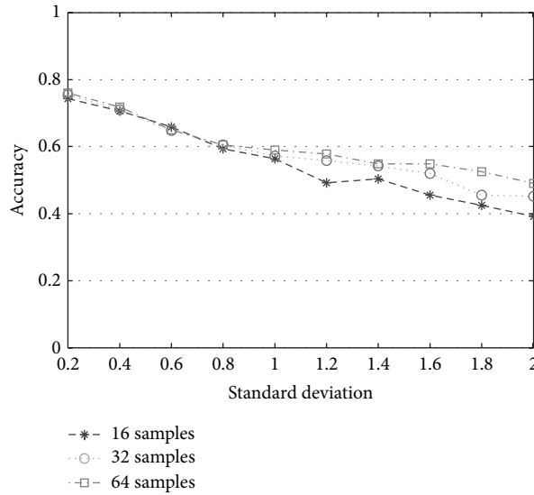
(c) Accuracy of 16, 32, and 64 sample observations with Exponential error
