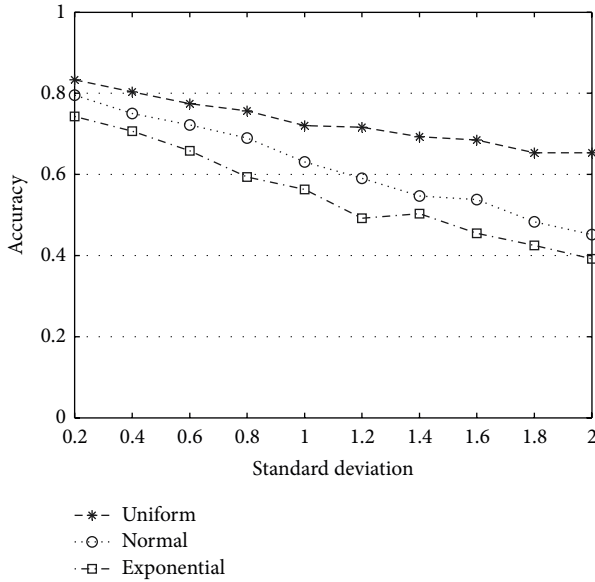
FIGURE 9: Accuracy with three error distributions averaged over all datasets.
