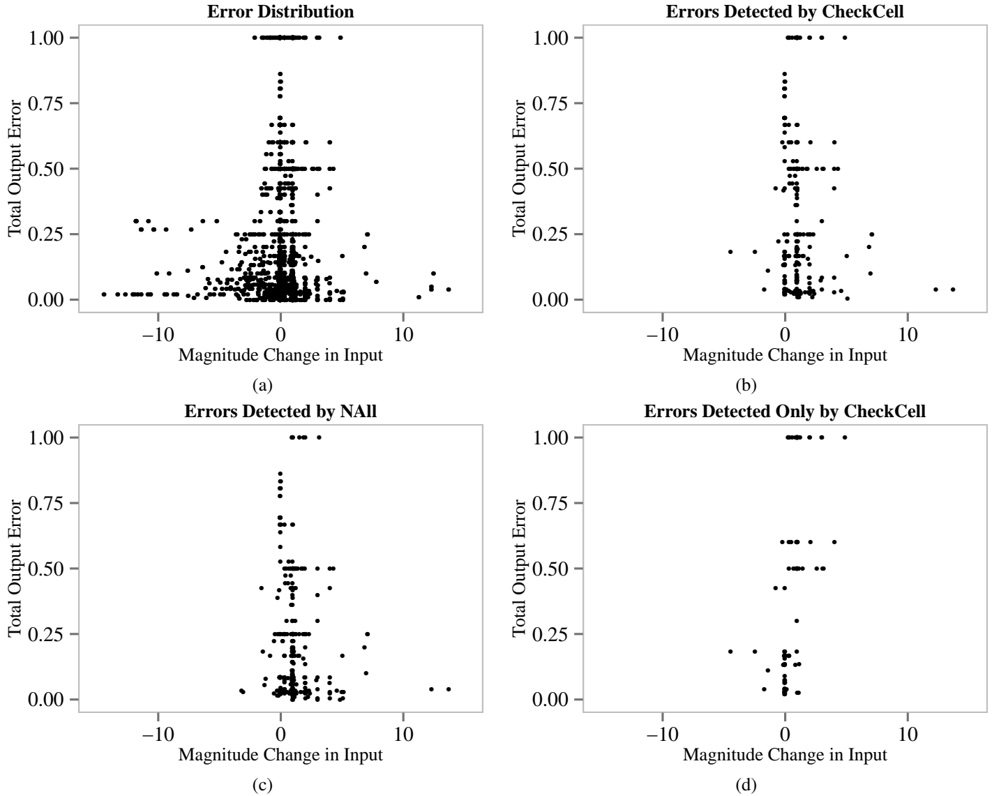
Figure 5. (a) The distribution of input errors. Each point corresponds to a single benchmark run. The change in input magnitude as the result of the error is shown on the x-axis while the change in the spreadsheet’s total error is shown on the y-axis. Note that because our typo generator was designed to produce representative errors, they are largely biased toward small-magnitude perturbations. (b) The distribution of errors caught by CC10. CHECKCELL favors errors that produce a large effect on the output. (c) The distribution of errors caught by NA11. NA11 favors large input errors in the input. (d) The distribution of errors found by CC10 but not by NA11. These errors tend to be subtle: they have a high impact on the spreadsheet’s output and are the result of small magnitude changes in the input.
