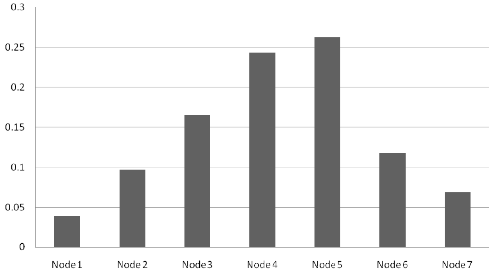
Figure 2: Distribution of Centipede Game Stopping Nodes
