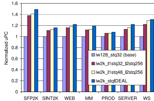
Figure 8. Hierarchical store queue performance
