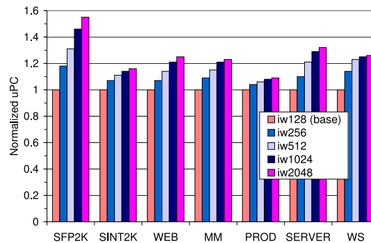
Figure 1. Impact of instruction window size
