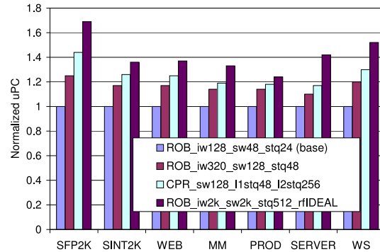
Figure 10. CPR performance.
