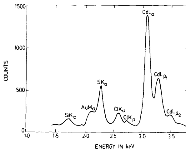
Figure 3. EDAX spectrum of a typical as deposited CdS thin film.
