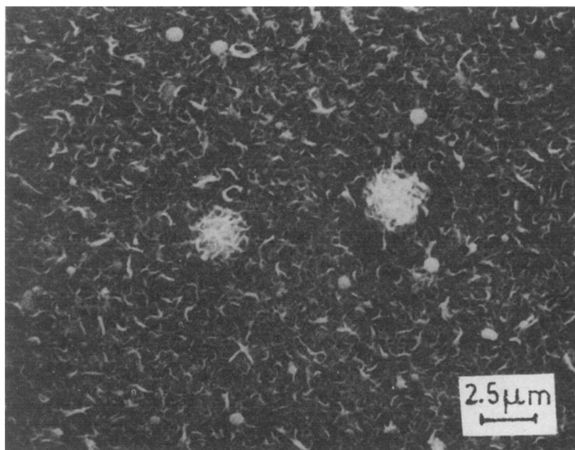
Figure 2. Scanning electron micrograph of as deposited CdS thin film.
