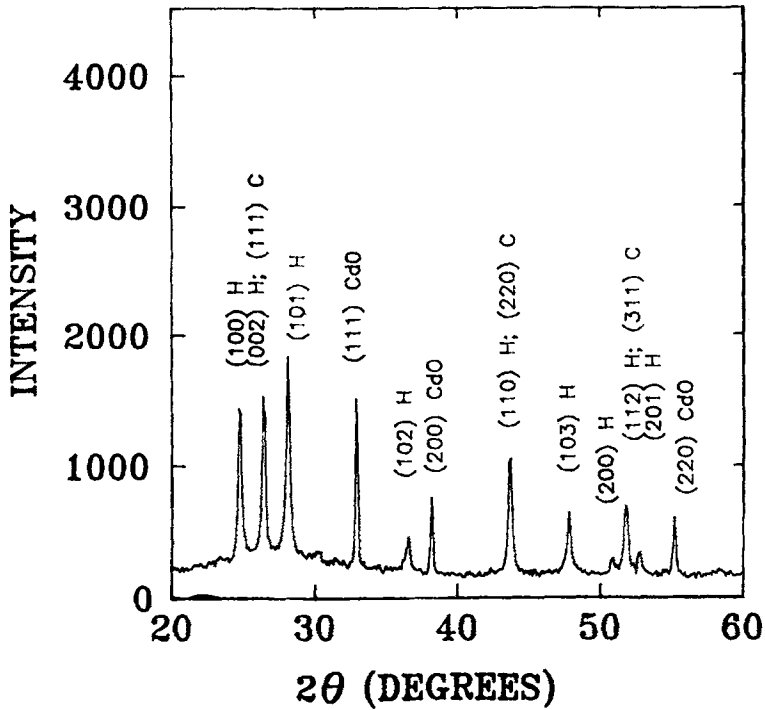
Figure 7. X-ray diffraction pattern of CdS thin film annealed in oxygen deficient atmosphere for 2 h at 673 K.
