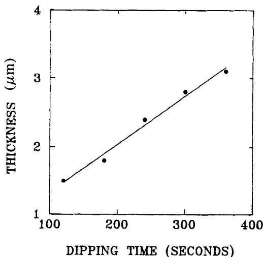
Figure 1. The figure shows the linear variation of film thickness with dipping time.
