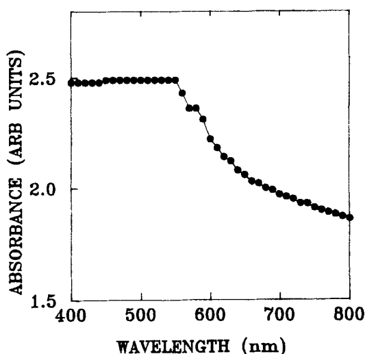
Figure 8. Optical absorption spectrum recorded for the typical annealed CdS thin film. It can be seen that the absorbance has increased considerably on annealing.
