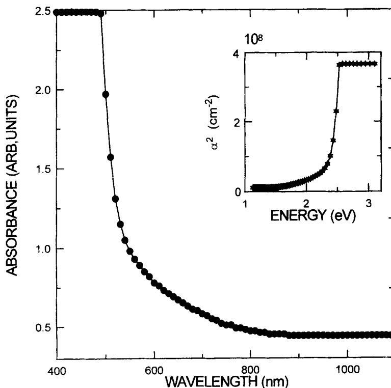
Figure 5. Optical absorption spectrum of as deposited CdS thin film (inset shows the plot of (\alpha)^2 versus h\nu ).
