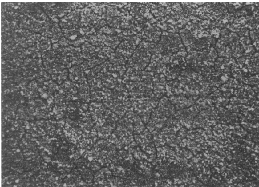
Figure 9. Scanning electron micrograph of annealed CdS thin film. It can be seen from the micrographs that the cracks are developed on annealing. These cracks are responsible for higher absorbance values.
