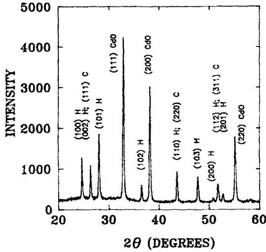
Figure 6. X-ray diffraction pattern of CdS thin film annealed in flowing air atmosphere for 2 h at 673 K.
