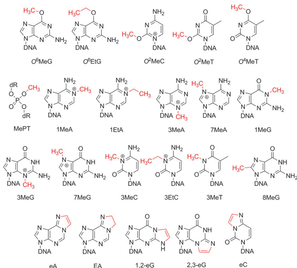
Fig. 3. Structures of DNA alkylation lesions.
