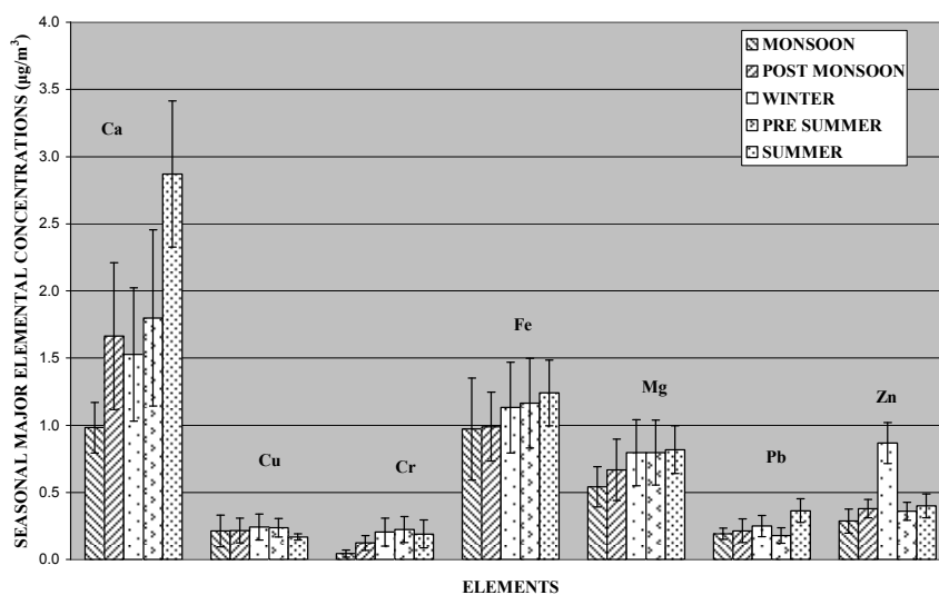
Fig. 3. Seasonal average major elemental concentrations.
