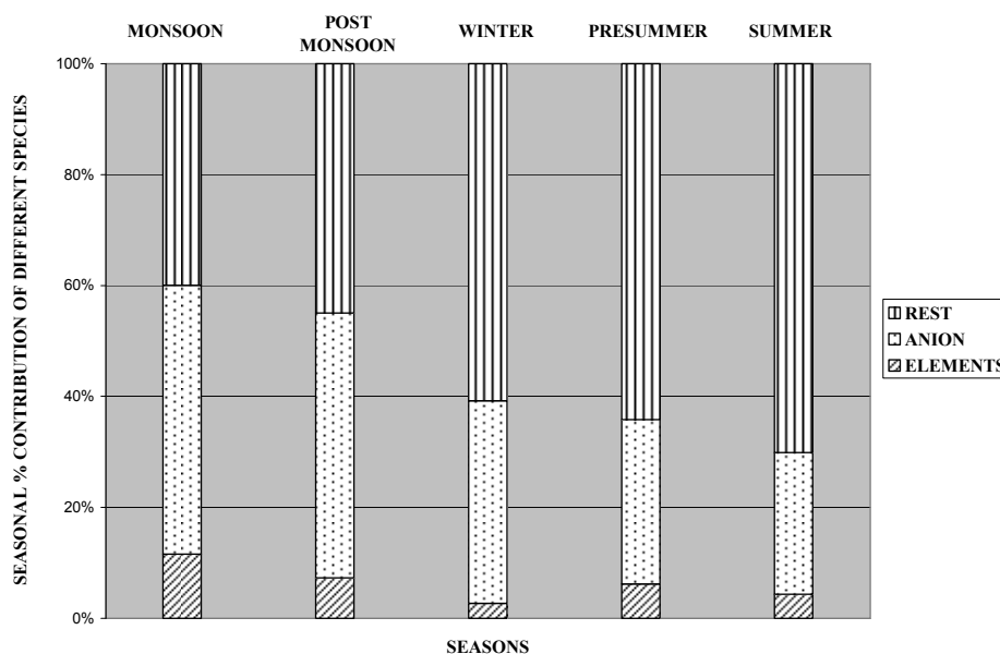
Fig. 8. % contribution of different species in seasonal PM 1 mass.
