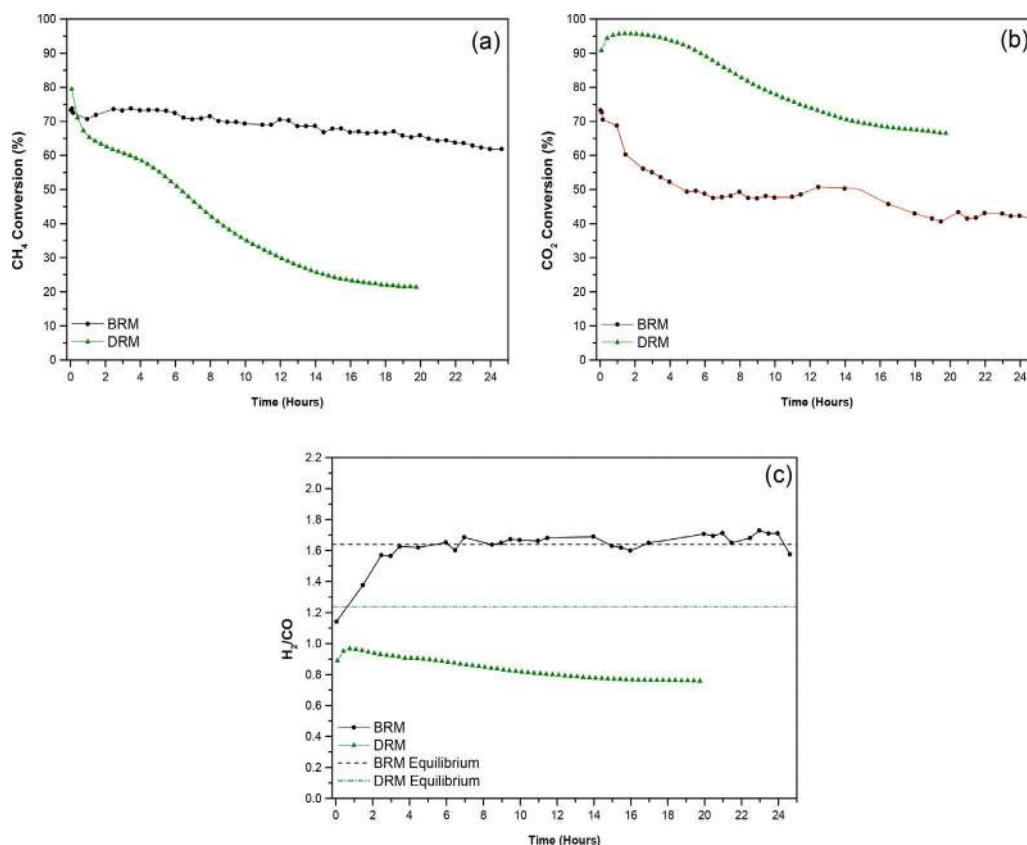
Fig. 11. Comparison of DRM ( \text{CH}_4/\text{CO}_2 = 1 ) and BRM ( \text{CH}_4/\text{CO}_2/\text{H}_2\text{O} = 1/1/1 ) for \text{Sn}_{0.02}\text{Ni}/\text{Ce-Al} at 700 °C and WHSV of 60,000 ml/(g-cat h): (a) Methane conversion; (b) \text{CO}_2 conversion; (c) \text{H}_2/\text{CO} ratio.
