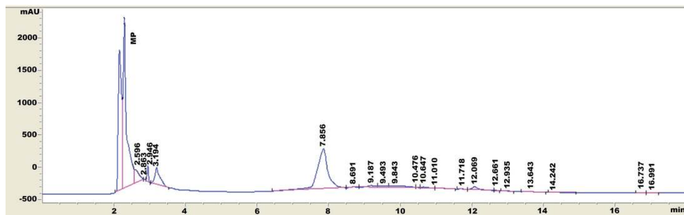
FIGURE 1 - Enlarged HPLC chromatogram of methanolic fraction obtained from Lepista sordida .
