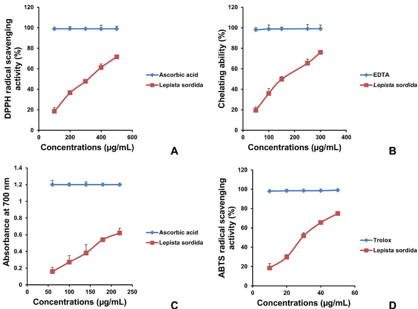
FIGURE 2 - Antioxidant activity of methanolic extract from Lepista sordida A) DPPH radical scavenging activity B) Chelating ability C) Reducing power D) ABTS radical scavenging activity.
