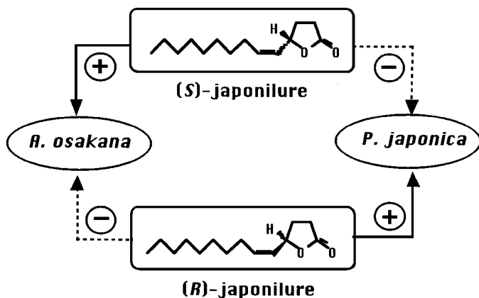
Figure 2 Schematic view of the mechanism of reciprocal behavioral agonist-antagonist activities of chiral pheromones.
