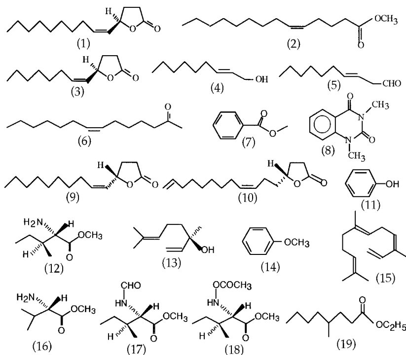
Figure 1 Semiochemicals involved in chemical communication of scarab beetles. (1) ( R,Z )-5-(—)-(1-decenyl)oxacyclopentan-2-one; (2) methyl 5-( Z )-tetradecenoate; (3) ( R,Z )-5-(—)-(1-octenyl)oxacyclopentan-2-one; (4) 2-( E )-nonenol; (5) 2-( E )-nonenal; (6) 7-( Z )-tetradecen-2-one; (7) methyl benzoate; (8) 1,3-dimethyl-2,4-(1 H ,3 H )-quinazolin-2(1 H )-one; (9) ( S,Z )-5-(+)-(1-decenyl)oxacyclopentan-2-one; (10) ( R,Z )-7,15-hexadecadien-4-olide; (11) phenol; (12) L -isoleucine methyl ester; (13) ( R )-(—)-linalool; (14) anisole; (15) ( Z,E )- \alpha -farnesene; (16) L -valine methyl ester; (17) N -formyl L -isoleucine methyl ester; (18) N -acetyl L -isoleucine methyl ester; (19) ethyl 4-methyloctanoate.
