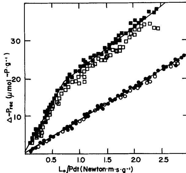
FIGURE 1. The relationship between total recovery chemical input and the tension-time integral. The recovery chemical input ( \Delta \sim P_{\text{rec}} ) is expressed in \mu\text{mol} \sim P/\text{g} and obtained from the following equation: \Delta \sim P_{\text{rec}} = \kappa \xi O_2 + \lambda \xi \text{lac} , where \kappa and \lambda are stoichiometric factor equal to 6.3 and 1.5, respectively. Open symbols represent the contribution to the total recovery chemical input from oxygen consumption alone ( \kappa \xi O_2 ) in the soleus ( \circ ) and EDL ( \square ). Closed symbols represent the total recovery chemical input after the contribution from glycolytic ATP production ( \lambda \xi \text{lac} ) was added to the aerobic contribution in soleus ( \bullet ) and EDL ( \blacksquare ). In a majority of the data points for the soleus, the contribution from lactate production was negligible, and for the sake of visual clarity only the points corresponding to the total recovery input were graphed. The lines are linear functions fitted to the data with the following parameters:
