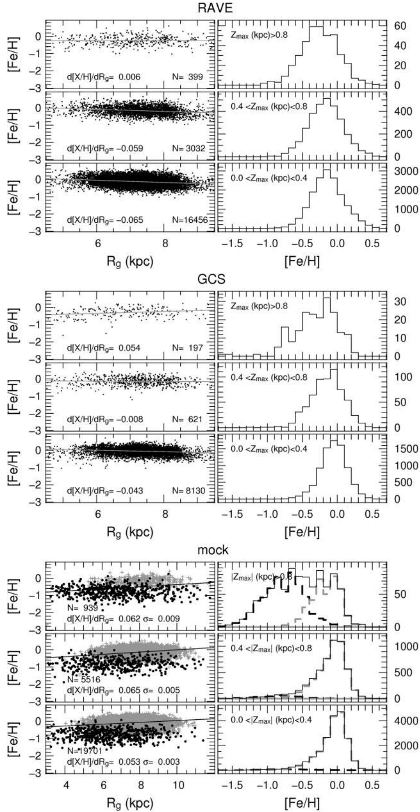
Fig. 3. Distributions of the dwarf stars for the RAVE sample ( top ), GCS sample ( middle ) and mock sample ( bottom ) in the ([Fe/H], R_g) planes ( left panels ) and [Fe/H] distributions ( right panels ). The grey line has a slope equal to the gradient. For the mock sample ( bottom ) grey plus symbols, black circles, and grey squares represent thin-disc, thick-disc, and halo stars, respectively. The same order is followed by the grey dashed, black dashed, and grey solid lines in the right panels , which represent the iron distributions of these subsamples.
