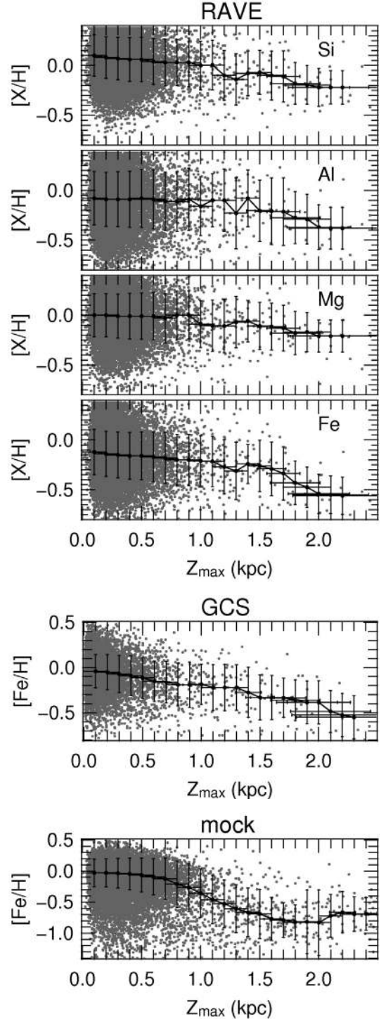
Fig. 5. Abundance for the elements Fe, Mg, Al, and Si for the RAVE sample ( top ), [Fe/H] for the GCS sample ( middle ) and the mock sample ( bottom ) as a function of Z_{\max} . The black dots connected by a line represent the median abundance. The vertical error bars indicate the standard deviation of the distribution computed in the Z_{\max} interval indicated by the horizontal error bars.
