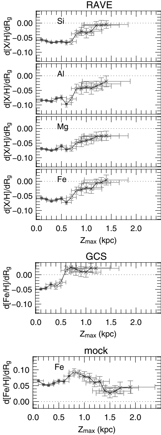
Fig. 4. Abundance gradients for Fe, Mg, Al and Si for the RAVE sample ( top ), [Fe/H] for GCS sample ( middle ), and for the mock sample ( bottom ) as a function of Z_{\max} . Horizontal error bars indicate the Z_{\max} interval in which the gradient has been measured. Vertical error bars indicate the gradient error estimated with the bootstrap technique outlined in Sect. 3.2. Full points indicate that the gradient has been computed with a sample containing N > 1000 stars; open square represent samples with 1000 < N < 300 stars; cross symbols represent samples with 200 < N < 300 stars.
