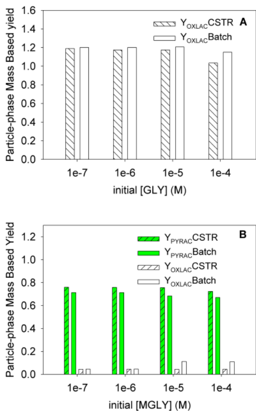
Fig. 10. The CSTR simulation and the batch simulation for particle-phase mass-based yields of oxalate ( Y_{\text{OXLAC}} ) with increasing initial concentrations of glyoxal for glyoxal + OH. (B) The CSTR simulation and the batch simulation for particle-phase mass-based yields of pyruvate ( Y_{\text{PYRAC}} ) and oxalate ( Y_{\text{OXLAC}} ) with increasing initial concentrations of methylglyoxal for methylglyoxal + OH.
