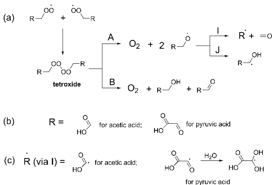
Fig. 1. Mechanism for peroxy radical reactions (a). The pathway A is suggested by Benson (1965), forming alkoxy radicals, followed by decomposition (I) or 1,2-hydride shift (J). The pathway B forming no organic radical product (i.e., B is a concerted reaction) is suggested by Russell et al. (1957). Parent precursors can be acetic acid or pyruvic acid (b). Fragmented organic radicals ( R^{\cdot} ) are expected to be stabilized by a carboxylic group for acetic acid ((c) left) and a diol, which results from hydration of a carbonyl group for pyruvic acid ((c) right).
