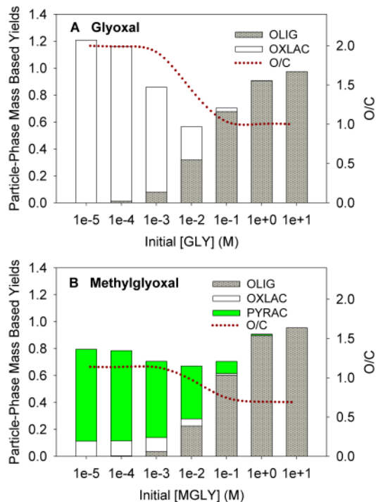
Fig. 9. Atmospheric batch simulations (A) for particle-phase mass-based yields of oxalate ( Y_{\text{OXLAG}} ), oligomers ( Y_{\text{OLIG}} ), and SOA ( = Y_{\text{OXLAG}} + Y_{\text{OLIG}} ) with increasing initial concentrations of glyoxal ( x axis) for aqueous-phase OH radical reactions, and (B) for particle-phase mass-based yields of oxalic acid ( Y_{\text{OXLAG}} ), pyruvate ( Y_{\text{PYRAC}} ), oligomers ( Y_{\text{OLIG}} ), and SOA ( = Y_{\text{OXLAG}} + Y_{\text{PYRAC}} + Y_{\text{OLIG}} ) with increasing initial concentrations of methylglyoxal ( x axis) for aqueous-phase OH radical reactions. Similarly, O/C (on the right-hand y axis) vs. initial concentrations of glyoxal (A) and O/C vs. initial concentrations of methylglyoxal (B).
