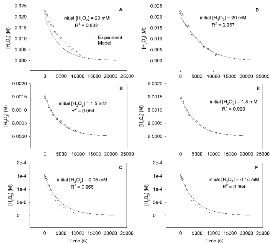
Fig. 4. Real-time profiles of 254 nm UV photolysis decay of \text{H}_2\text{O}_2 (where initial concentrations are 0.15, 1.5, and 20 mM) without light-absorption correction (A, B, and C) and with the correction (D, E, and F). The correction was made by multiplying the transmittance by the \text{H}_2\text{O}_2 photolysis decay rate constant, where -\log(\text{transmittance}) = 18.4 \times 0.80 \times [\text{H}_2\text{O}_2] .
