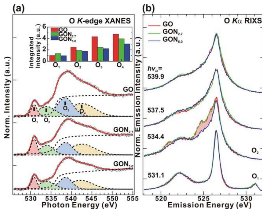
Figure 4. (a) O 1s XANES and de-convoluted features. The inset is the intensity bar diagram of O 1s XANES features of GO and GO:N x (x = 2.7 and 5.0), obtained by fitting. (b) O K α RIXS spectra of GO and GO:N x (x = 2.7 and 5.0).
