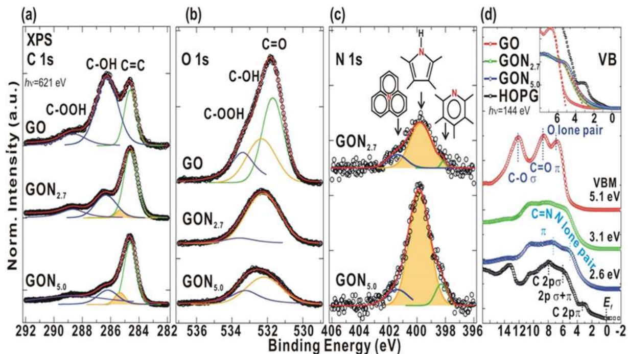
Figure 2. (a) C 1s, (b) O 1s and (c) N 1s XPS of GO and GO: N_x ( x = 2.7 and 5.0 ), respectively. Open circles represent measured spectra, and red solid curves represent fitting results. Each solid curve is fitted using Voigt-shaped function following background subtraction. (d) Valence-band of GO, GO: N_x ( x = 2.7 and 5.0 ) and HOPG. Inset (d) magnifies the region of VBM or E_f of GO, GO: N_x ( x = 2.7 and 5.0 ) and HOPG.
