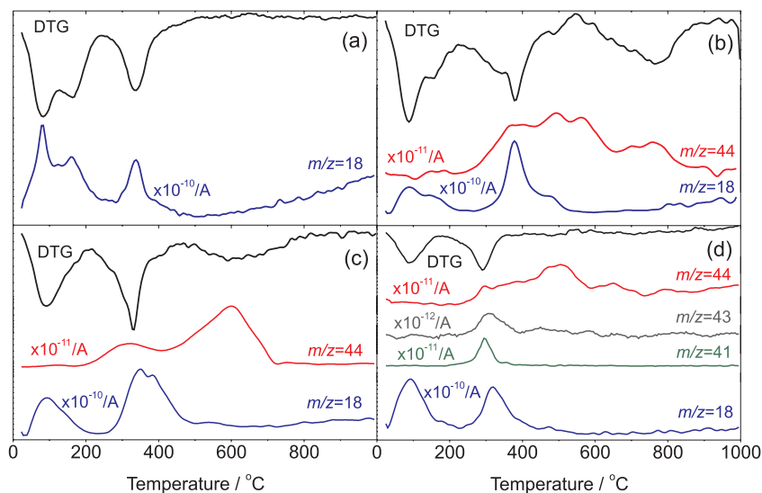
Figure 8. DTG-MS curves of (a) \text{H}_2\text{K}_2\text{Nb}_6\text{O}_{17} , (b) \text{tma}(0.50)\text{dep} , (c) \text{tea}(0.50)\text{dep} and (d) \text{tpa}(0.50)\text{dep} .
