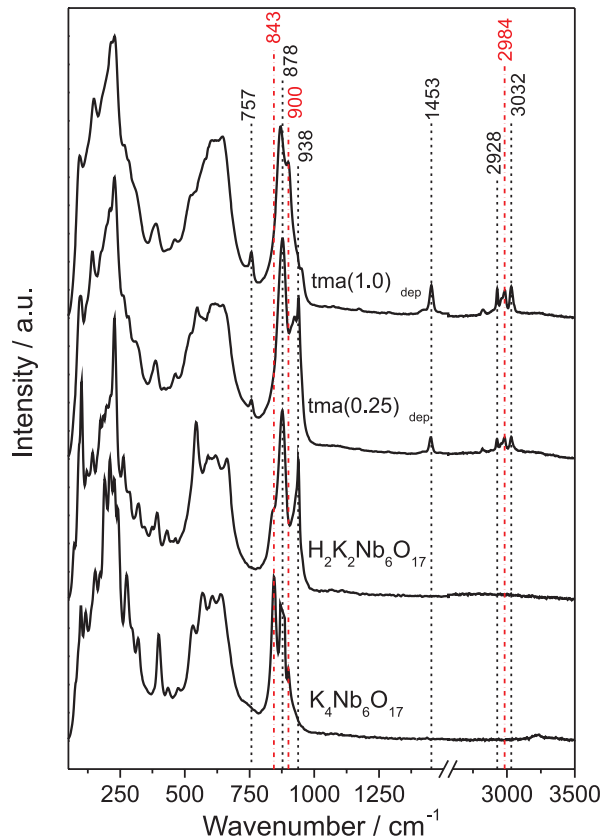
Figure 6. FT-Raman spectra of K_4Nb_6O_{17} , H_2K_2Nb_6O_{17} , tma(0.25)dep and tma(1.0)dep.
