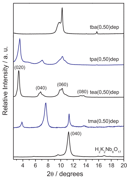
Figure 3. XRD patterns of \text{H}_2\text{K}_2\text{Nb}_6\text{O}_{17} , \text{tma}(0.50)\text{dep} , \text{tea}(0.50)\text{dep} , \text{tpa}(0.50)\text{dep} and \text{tba}(0.50)\text{dep} .
