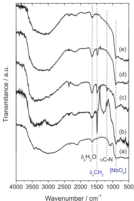
Figure 5. FTIR spectra of (a) \text{H}_2\text{K}_2\text{Nb}_6\text{O}_{17} , (b) tma(0.50)dep, (c) tea(0.50)dep, (d) tpa(0.50)dep and (e) tba(0.50)dep.
