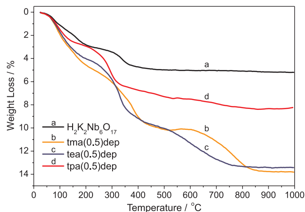
Figure 7. TGA curves of H_2K_2Nb_6O_{17} , tma(0.5)dep, tea(0.5)dep and tpa(0.5)dep.
