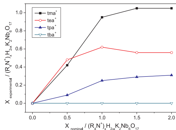
Figure 2. Experimental versus nominal values of X in the general formula (\text{R}_4\text{N}^+)_x\text{H}_{2-2x}\text{K}_2\text{Nb}_6\text{O}_{17} , where \text{R}_4\text{N}^+ = tetraalkylammonium cation.
