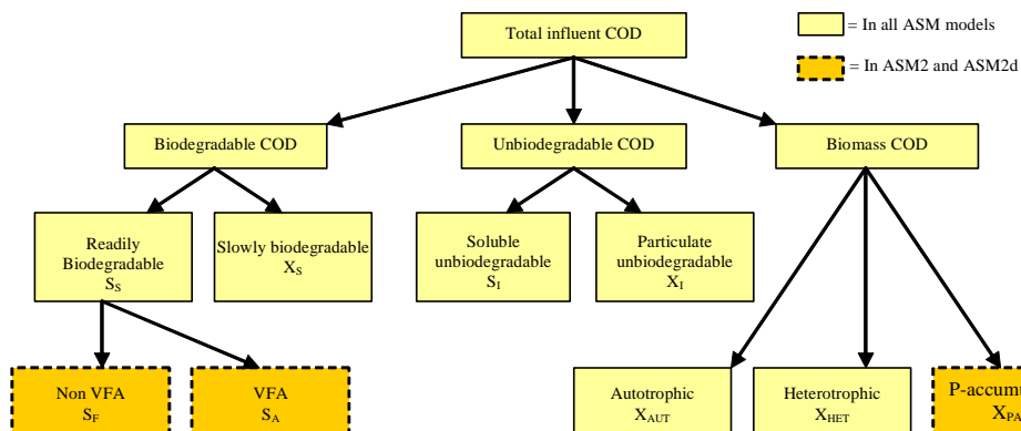
Fig. 1: Division of influent wastewaters into COD components in ASM model family
