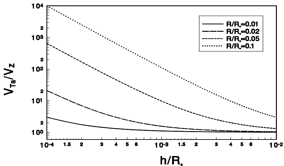
FIG. 34 Plot of V_{Ta}/V_z vs. h/R_* for various values of the dimensionless film radius, R/R_* . V_{Ta} corresponds to two nondeformed (spherical) particles (Equation 260), whereas V_z is the velocity of approach of two deformed particles (Eq. 259).
