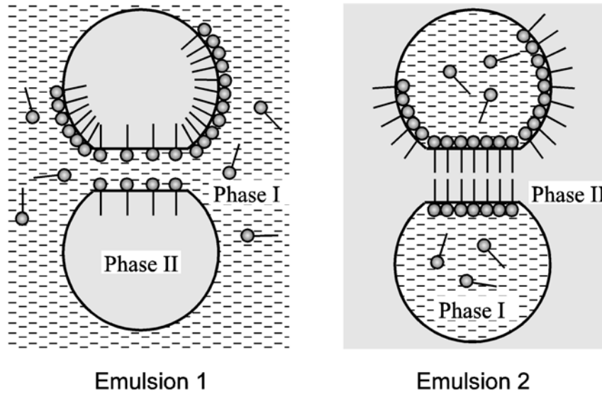
FIGURE 44. The two possible types of emulsions obtained just after the homogenization; the surfactant is soluble into Phase I.
