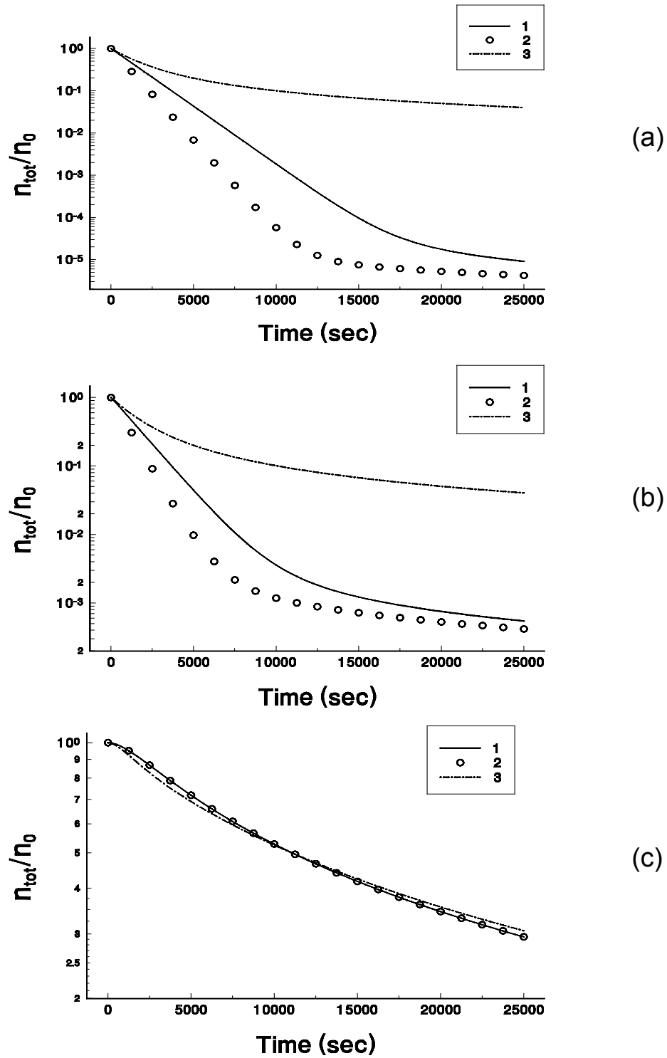
FIGURE 56 Relative change in the total number of drops, n_{tot} , vs. time, t ; initial number of primary drops n_0 = 10^{12} cm -3 ; coalescence rate constant k_c^{2,1} = 10^{-3} sec -1 . Curve 1: numerical solution of Equation 336; curve 2: output of the model of Borwankar et al., 671 curve 3: output of the model of van den Tempel, 670 the values of the flocculation rate constant are (a) a_f = 10^{-11} cm 3 /s; (b) a_f = 10^{-13} cm 3 /s; (c) a_f = 10^{-16} cm 3 /s.
