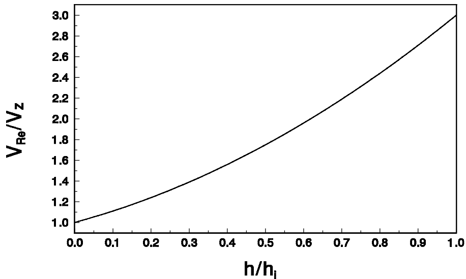
FIG. 33 Plot of V_{Re}/V_z vs. h/h_i for two fluid particles (Equation 259) which are deformed because of the viscous friction in the transition zone between the film and the bulk phase (see Figure 32).
