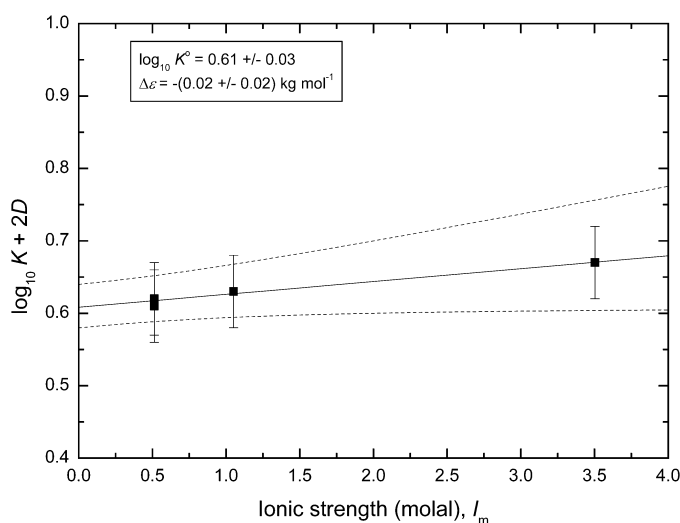
Fig. A3-4 Extrapolation to I = 0 of \log_{10} K - \Delta(z^2)D for reaction 10 using selected data for (\text{Na,H})\text{ClO}_4 media at \text{pH} \approx 2 ( \text{pH} \approx 1.3 in [68CGb]), 25 °C (Table A2-5). The error bounds are derived by using the uncertainty ranges of \log_{10} K^\circ and \Delta\varepsilon to recalculate \log_{10} K(I_m) up to I_m = 4 \text{ mol kg}^{-1} .
