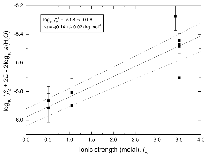
Fig. A3-2 Extrapolation to I = 0 of \log_{10} {}^*\beta_2 - \Delta(z^2)D - 2\log_{10} a(\text{H}_2\text{O}) for reaction 5 using selected data for \text{NaClO}_4 and \text{CaClO}_4 media, 25 °C (Table A2-2). The error bounds are derived by using the uncertainty ranges of \log_{10} {}^*\beta_2^\circ and \Delta\epsilon to recalculate \log_{10} {}^*\beta_2(I_m) up to I_m = 4 \text{ mol kg}^{-1} .
