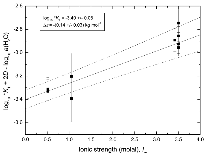
Fig. A3-1 Extrapolation to I = 0 of \log_{10} {}^*K_1 - \Delta(z^2)D - \log_{10} a(\text{H}_2\text{O}) (eq. 3, Section 5.2) for reaction 4 using selected data for \text{NaClO}_4 solution, 25 °C, Table A2-1. The error bounds are derived by using the uncertainty ranges of \log_{10} {}^*K_1^\circ and \Delta\epsilon to recalculate \log_{10} {}^*K_1(I_m) up to I_m = 4 \text{ mol kg}^{-1} .
