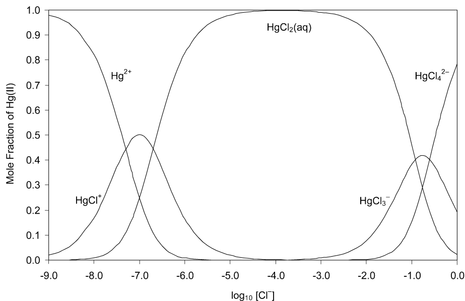
Fig. 2 Speciation diagram of the binary Hg(II) chloride system as obtained from the Recommended stability constants at I_m = 0 \text{ mol kg}^{-1} , Table 2. Hydrolysis is suppressed ( \text{pH} < 2 is assumed). Results for -\log [\text{Cl}^-] > -2.0 should be viewed with caution as activity coefficients deviate from 1.0.
