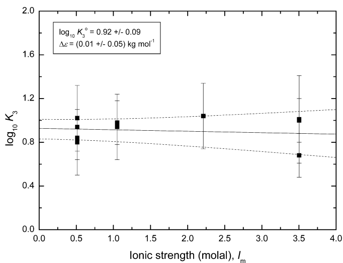
Fig. A3-6 Extrapolation to I = 0 of \log_{10} K_3 for reaction 8 ( \Delta(z^2)D = 0 ) using selected data for \text{NaClO}_4 media containing varying and significant proportions of \text{Cl}^- ; 25 °C (Table A2-7) The error bounds are derived by using the uncertainty ranges of \log_{10} K_3^0 and \Delta\epsilon to recalculate \log_{10} K_3(I_m) up to I_m = 4 \text{ mol kg}^{-1} .
