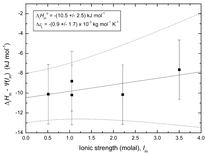
Fig. A3-13 Extrapolation to I = 0 of the enthalpy for reaction 9 in \text{NaClO}_4 solutions containing varying and significant proportions of \text{Cl}^- ; 25 °C (Table A2-15). The error bounds are derived by using the uncertainty ranges of \Delta H_m^\circ and \Delta \epsilon_L to recalculate \Delta H_m to I_m = 4 \text{ mol kg}^{-1} .
