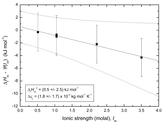
Fig. A3-12 Extrapolation to I = 0 of the enthalpy for reaction 8 in \text{NaClO}_4 solutions containing varying and significant proportions of \text{Cl}^- ; 25^\circ\text{C} (Table A2-15). The error bounds are derived by using the uncertainty ranges of \Delta_r H_m^\circ and \Delta \epsilon_L to recalculate \Delta_r H_m to I_m = 4 \text{ mol kg}^{-1} .
