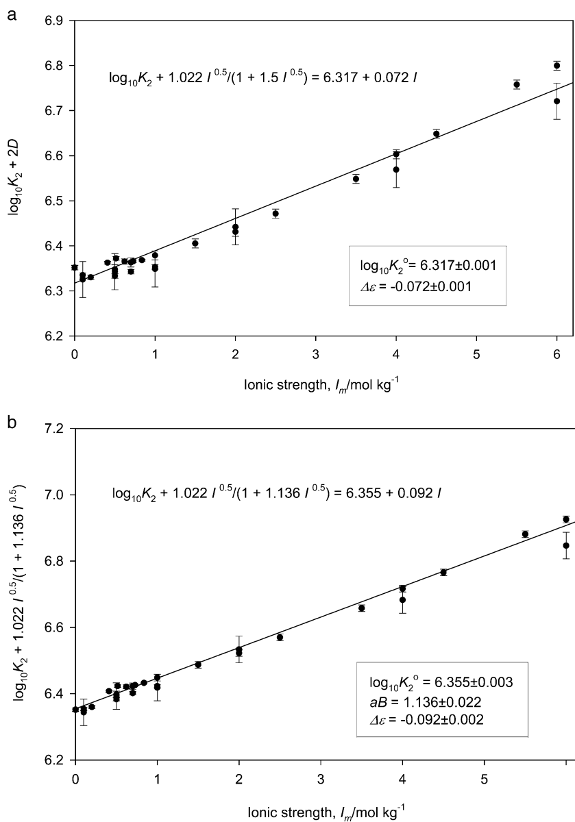
Fig. A4-2 Extrapolation to I_m = 0 \text{ mol kg}^{-1} of \log_{10} K_2 - \Delta(z^2)D for reaction 23, using the selected data for NaCl media, 25 °C (Table A4-1a). The regression uses eq. 3 with a(\text{H}_2\text{O}) equal to unity. Figure (a) assumes a_i B = 1.5 \text{ kg}^{1/2} \text{ mol}^{-1/2} . Figure (b) treats a_j B in the term D (eq. 1) as an empirical parameter, which refines to 1.136 \text{ kg}^{1/2} \text{ mol}^{-1/2} .
