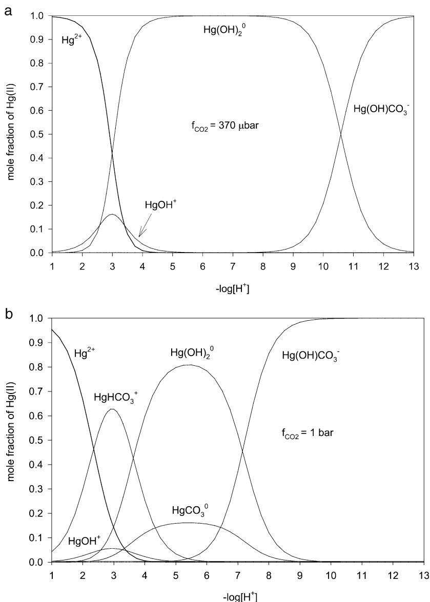
Fig. 3 Speciation diagrams for the \text{Hg}^{2+} – \text{H}^+ – \text{CO}_2 system as obtained from the selected stability constants reported in Tables 1 and 3 and calculated for (a) f(\text{CO}_2) = 370 microbar and (b) f(\text{CO}_2) = 1 bar. These diagrams are applicable for \text{Hg}(\text{II}) concentrations below \leq 0.01 \text{ mmol dm}^{-3} . Results outside the -\log [\text{H}^+] range of 2 to 12 should be viewed with caution as activity coefficients deviate from 1.0.
