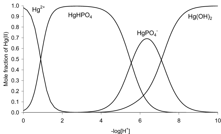
Fig. 4 Speciation diagram for the \text{Hg}^{2+} - \text{H}^+ - \text{PO}_4^{3-} system (total concentrations [\text{Hg}^{2+}]_{\text{T}} = 5 \times 10^{-5} \text{ mol dm}^{-3} and [\text{PO}_4^{3-}]_{\text{T}} = 5 \times 10^{-3} \text{ mol dm}^{-3} ) as obtained from the selected stability constants reported in Table 4 ( I_c = 3 \text{ mol dm}^{-3} \text{ NaClO}_4 ).
