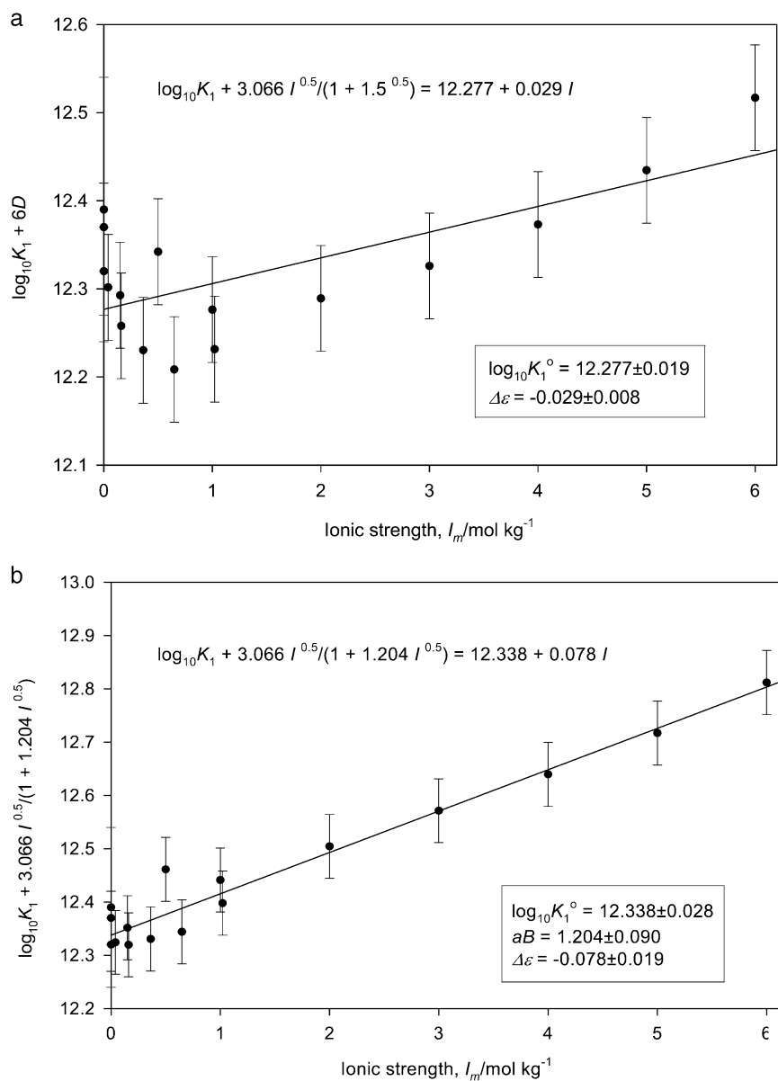
Fig. A4-3 Extrapolation to I_m = 0 \text{ mol kg}^{-1} of \log_{10} K_1 - \Delta(z^2)D for reaction 24, using the selected data for NaCl media, 25 °C (Table A4-2). The regression uses eq. 3 with a(\text{H}_2\text{O}) equal to unity. Figure (a) assumes a_j B = 1.5 \text{ kg}^{1/2} \text{ mol}^{-1/2} . Figure (b) treats a_j B in the term D (eq. 1) as an empirical parameter, which refines to 1.204 \text{ kg}^{1/2} \text{ mol}^{-1/2} .
