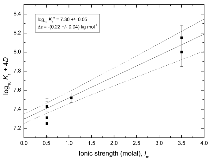
Fig. A3-3 Extrapolation to I = 0 of \log_{10} K_1 - \Delta(z^2)D for reaction 6 using selected data (Table A2-4) at 25 °C for \text{NaClO}_4 media, \text{pH} \approx 2 ( \text{pH} \approx 1.3 in [68CGb], \text{pH} \approx 1 in [63H1a], \text{pH} variable in [77SJB]). The error bounds are derived by using the uncertainty ranges of \log_{10} K_1^\circ and \Delta\varepsilon to recalculate \log_{10} K_1(I_m) up to I_m = 4 \text{ mol kg}^{-1} .
