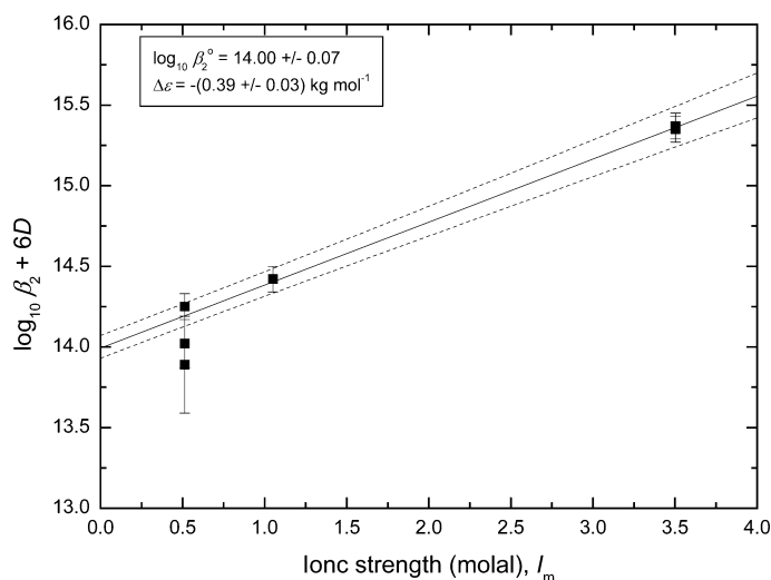
Fig. A3-5 Extrapolation to I = 0 of \log_{10} \beta_2 - \Delta(z^2)D for reaction 7 using selected data for \text{NaClO}_4 media, 25 °C (Table A2-6); pH \approx 1.3 in [68CGb], pH \approx 1 in [63Hla], pH variable in [77Sjb]. The error bounds are derived by using the uncertainty ranges of \log_{10} \beta_2^0 and \Delta\epsilon to recalculate \log_{10} \beta_2(I_m) up to I_m = 4 \text{ mol kg}^{-1} .
