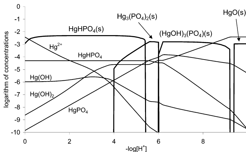
Fig. 5 Speciation diagram for soluble and insoluble species in the \text{Hg}^{2+} - \text{H}^+ - \text{PO}_4^{3-} system (total concentrations [\text{Hg}^{2+}]_{\text{T}} = 5 \times 10^{-3} \text{ mol dm}^{-3} and [\text{PO}_4^{3-}]_{\text{T}} = 5 \times 10^{-3} \text{ mol dm}^{-3} ) as obtained from the selected stability and solubility constants reported in Table 4 ( I_c = 3 \text{ mol dm}^{-3} \text{ NaClO}_4 ). Solid phases shown by bold lines.
