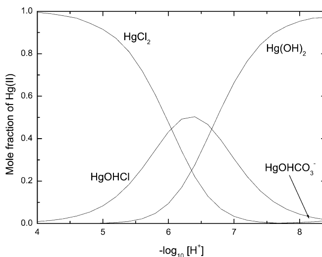
Fig. 6 Speciation diagram for the \text{Hg}^{2+} – \text{H}^+ – \text{Cl}^- – \text{CO}_2 – \text{HPO}_4^{2-} – \text{SO}_4^{2-} system with total concentrations [\text{Cl}^-]_{\text{T}} = 0.23 \text{ mmol dm}^{-3} , [\text{SO}_4^{2-}]_{\text{T}} = 0.42 \text{ mmol dm}^{-3} , and [\text{HPO}_4^{2-}]_{\text{T}} = 0.7 \text{ } \mu\text{mol dm}^{-3} . The total concentration of \text{Hg}(\text{II}) was set to 1 \text{ nmol dm}^{-3} , and it was assumed that the system was in equilibrium with air having a \text{CO}_2 fugacity of 370 \text{ } \mu\text{bar} . \text{Log } K_{10}[\text{CO}_2(\text{g}) \rightleftharpoons \text{CO}_2(\text{aq})] = -1.5 [93MOR]. All other formation constants are according to Tables 1 to 7.
