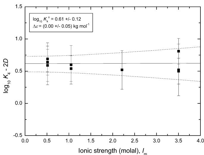
Fig. A3-7 Extrapolation to I = 0 of \log_{10} K_4 - \Delta(z^2)D for reaction 9 using selected data for \text{NaClO}_4 media containing varying and significant proportions of \text{Cl}^- ; 25 °C (Table A2-7). The error bounds are derived by using the uncertainty ranges of \log_{10} K_4^\circ and \Delta\varepsilon to recalculate \log_{10} K_4(I_m) up to I_m = 4 \text{ mol kg}^{-1} .
