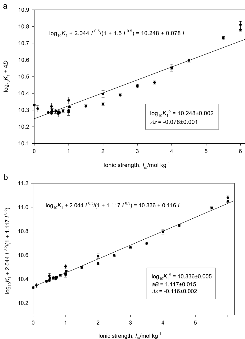
Fig. A4-1 Extrapolation to I_m = 0 \text{ mol kg}^{-1} of \log_{10} K_1 - \Delta(z^2)D for reaction 22, using the selected data for NaCl media, 25 °C (Table A4-1a). The regression uses eq. 3 with a(\text{H}_2\text{O}) equal to unity. Figure (a) assumes a_j B = 1.5 \text{ kg}^{1/2} \text{ mol}^{-1/2} . Figure (b) treats a_j B in the term D (eq. 1) as an empirical parameter, which refines to 1.117 \text{ kg}^{1/2} \text{ mol}^{-1/2} .
