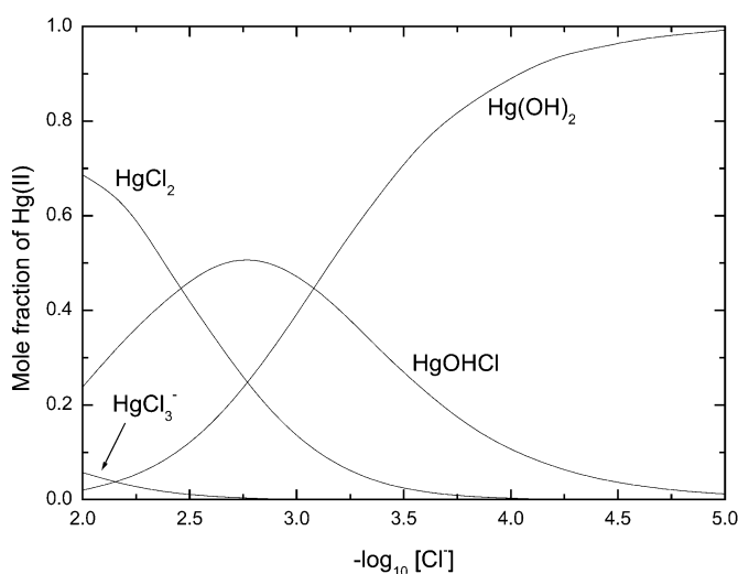
Fig. 7 Speciation diagram for the \text{Hg}^{2+} – \text{H}^+ – \text{Cl}^- – \text{CO}_2 – \text{HPO}_4^{2-} – \text{SO}_4^{2-} system. Concentrations as in Fig. 6 except for pH, which is kept constant at 7.22, and [\text{Cl}^-]_{\text{free}} which was allowed to vary between 10^{-5} and 10^{-2} mol \text{dm}^{-3} .
