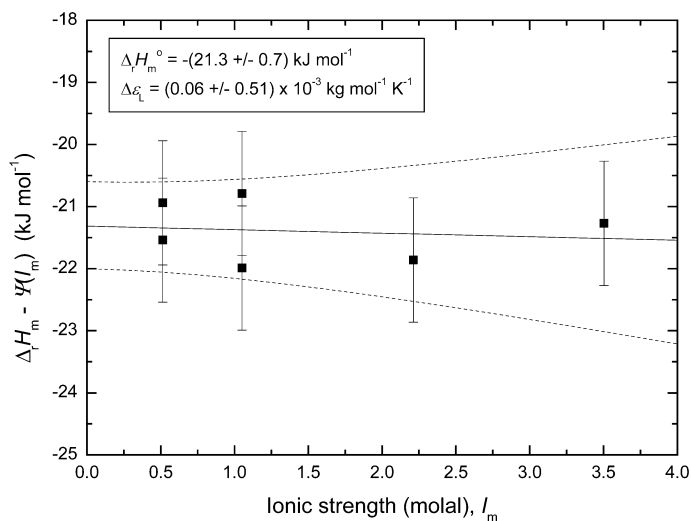
Fig. A3-10 Extrapolation to I = 0 of the enthalpy for reaction 6 in \text{NaClO}_4 solutions at \text{pH} \approx 2 [65ARa], \text{pH} \approx 1.3 [75CGe] and \text{pH} \approx 1 [64ClA, 80VKb]; 25^\circ\text{C} (Table A2-14). The error bounds are derived by using the uncertainty ranges of \Delta_r H_m^\circ and \Delta \epsilon_L to recalculate \Delta_r H_m up to I_m = 4 \text{ mol kg}^{-1} .
