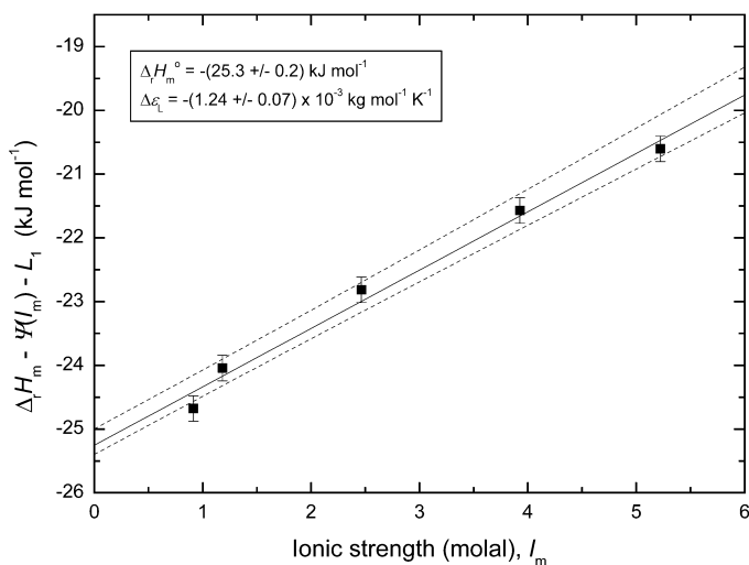
Fig. A3-8 Extrapolation of enthalpy data for reaction 29 to I = 0 , according to eq. 37; \text{HClO}_4 media, 25 °C (Table A2-13). The error bounds are derived by using the uncertainty ranges of \Delta_r H_m^\circ and \Delta\varepsilon_L to recalculate \Delta_r H_m(I_m) up to I_m = 6 \text{ mol kg}^{-1} .
