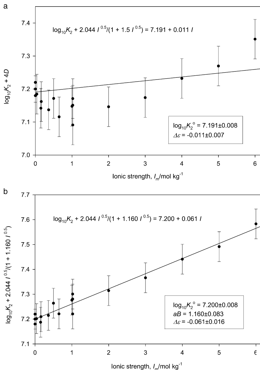
Fig. A4-4 Extrapolation to I_m = 0 \text{ mol kg}^{-1} of \log_{10} K_2 - \Delta(z^2)D for reaction 25, using the selected data for NaCl media, 25 °C (Table A4-2). The regression uses eq. 3 with a(\text{H}_2\text{O}) equal to unity. Figure (a) assumes a_j B = 1.5 \text{ kg}^{1/2} \text{ mol}^{-1/2} . Figure (b) treats a_j B in the term D (eq. 1) as an empirical parameter, which refines to 1.160 \text{ kg}^{1/2} \text{ mol}^{-1/2} .
