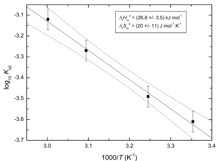
Fig. A3-9 Plot of \log_{10} K_{s2} for reaction 28 (HgO(yellow)) against absolute temperature. The slope of the regression line is -(\Delta_r H_m^\circ/2.303R) and the intercept (\Delta_r S_m^\circ/2.303R) . The error bounds are derived by using the uncertainty ranges of \Delta_r H_m^\circ and \Delta_r S_m^\circ to recalculate \log_{10} K_{s2}(T) .
