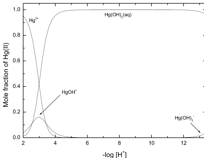
Fig. 1 Speciation diagram for the binary Hg(II) hydroxide system as obtained from the Recommended stability constants at I_m = 0 \text{ mol kg}^{-1} (Table 1). This diagram is applicable for Hg(II) concentrations \leq 0.01 \text{ mmol dm}^{-3} . Results outside the -\log [\text{H}^+] range of 2 to 12 should be viewed with caution as activity coefficients deviate from 1.0.
