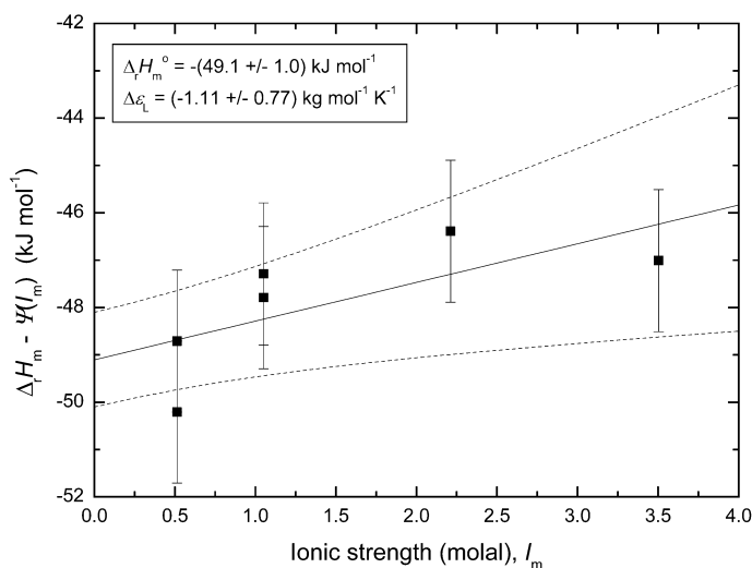
Fig. A3-11 Extrapolation to I = 0 of the enthalpy for reaction 7 in \text{NaClO}_4 solutions at \text{pH} \approx 2 [65ARa], \text{pH} \approx 1.3 [75CGe], and \text{pH} \approx 1 [64CIa, 80VKb]; 25^\circ\text{C} (Table A2-14). The error bounds are derived by using the resulting uncertainty ranges of \Delta_r H_m^\circ and \Delta \epsilon_L to recalculate \Delta_r H_m up to I_m = 4 \text{ mol kg}^{-1} .
