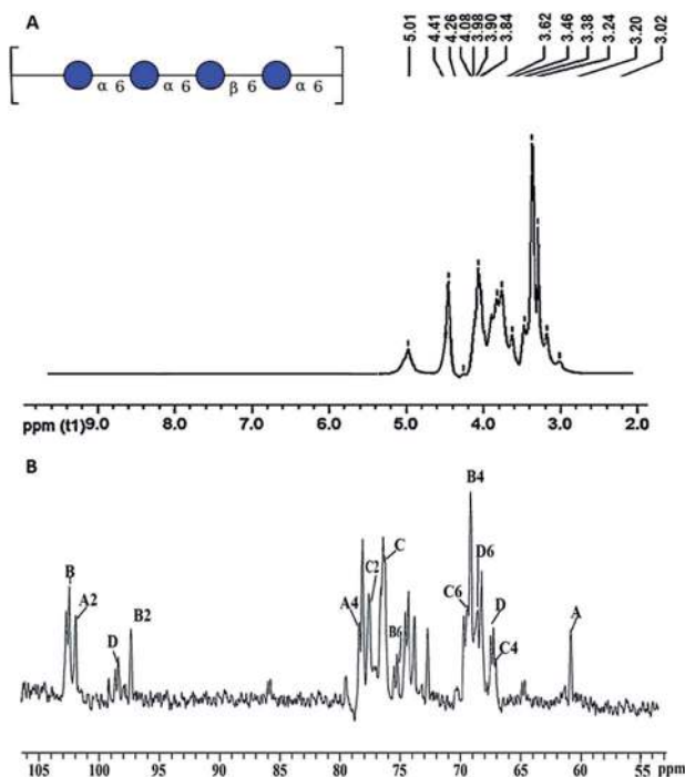
Fig. 4 NMR spectrum of the polysaccharide: (A) 1 H-NMR and (B) 13 C-NMR.
