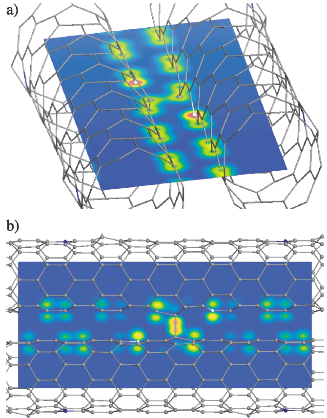
FIG. 3 (color). Two zigzag nanotubes each doped with nitrogen (white balls), facing each other. The chemical bond is formed between the two carbon atoms (grey balls), which have the maximum of the spin density in the isolated nanotube. The slice taken through the C-C bond shows the distribution of the (a) total charge density and (b) density of the HOMO orbital, using the color map, with blue corresponding to the lowest and red to the highest densities.
