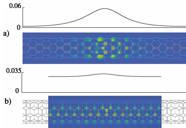
FIG. 1 (color). Slice of the spin density of the N-doped carbon nanotube in a plane parallel to the tube axis, the plane being tangential to the tube at the position of the nitrogen ion, for (a) (8,0) zigzag tube, comprising 12 unit cells (50.6 Å), and (b) (5,5) armchair tube, comprising 14 unit cells (34.3 Å). Above each slice, we plot the envelope of the spin density (integrated in the plane perpendicular to the tube) in the units of electron/Å. The nitrogen ion is marked white. The color range maps the value of the spin density, with blue corresponding to the smallest and red to the highest values. Note that the scale of the spin density is quite different for the two panels.
