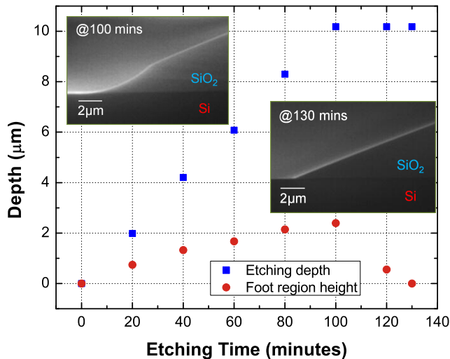
FIG. 4: Data plot showing the effect of etch time on appearance of the “foot” region in etching of a 10 micron thick silica layer. The foot region is a separate etch front produced by wet etch of silica that is empirically observed to adversely affect the optical Q factor. The data show that by control of the etch time the “foot” region can be eliminated. The upper-left inset is an image of the foot region and the lower right inset shows the foot region eliminated by increase of the wet etch time.
