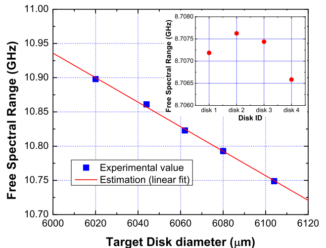
FIG. 3: Plot of measured free spectral range (FSR) versus the target design-value resonator diameter on a lithographic mask. The plot shows one device at each size and five different sizes. The rms variance is 2.4 MHz (relative variance of less than 1 : 4,500). The inset shows the FSR data measured on four devices having the same target FSR. An improved variance of 0.45 MHz is obtained (a relative variance of 1 : 20,000).
