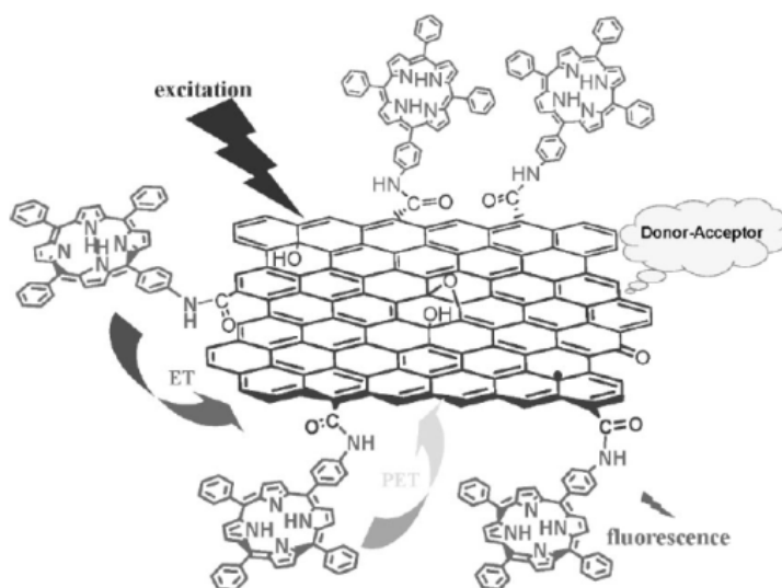
Figure 7. Chemical functionalization of graphene using amidation reaction (Adv. Maters. 2009;21(4) 1275-1279.)
