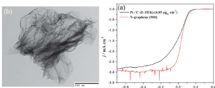
Figure 9. TEM image of nitrogen doped graphene and its electrochemical performance as a metal free catalyst for ORR. (Energy & Environ. Sci. 2011;4(3) 760-764.)
