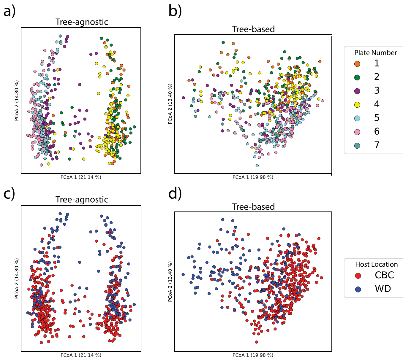
Extended Data Fig. 6 | Qemistree mitigates plate-to-plate variation in fecal metabolomics study to highlight a biologically-relevant effect. a) Principal coordinate analysis (PCoA) of tree-agnostic distances (Bray-Curtis) colored by plate number (pseudo-F = 32.39, p = 0.001 ). b) PCoA of tree-informed distances (Weighted UniFrac) colored by plate number (pseudo-F = 15.67, p = 0.001 ). The same PCoA of c) Bray-Curtis distances (pseudo-F = 33.50, p = 0.001 ) and d) Weighted UniFrac distances (pseudo-F = 48.42, p = 0.001 ) colored by cheetah location which governed the diet of cheetahs. CBC: Cheetah Breeding Center; WD: Wildlife Discoveries.
