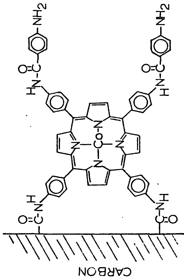
C\sim Co(NH_2)_4TPP
