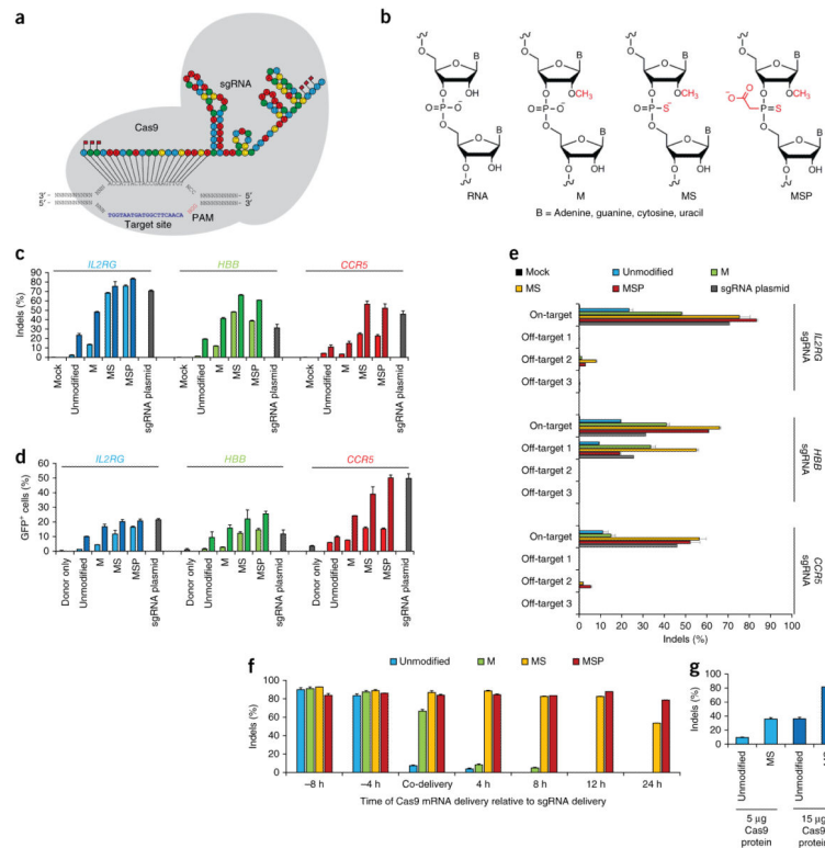
Figure 1. Synthesized and chemically modified sgRNAs facilitate high frequencies of indels and HR in the human cell line K562. (a) Sequence and schematic secondary structure of the IL2RG sgRNA loaded into Cas9 and bound to its genomic target site. Nucleotides with chemical modifications are marked with red flags. (b) Structures of chemical modifications incorporated during chemical synthesis of sgRNAs (sequences can be found in Supplementary Table 1 ). (c,d) amplicons (c) or gene addition by HR at the three loci IL2RG , HBB and CCR5 with synthetic sgRNAs (d) . The synthetic sgRNAs were delivered at 1 \mu g (light shade) or 20 \mu g (dark shade) per 1 million cells. Cas9 was expressed from a plasmid (2 \mu g) and for HR experiments 5 \mu g of GFP-encoding donor plasmid was included. As a positive control, 2 \mu g of sgRNA plasmid encoding both the sgRNA and the Cas9 protein was used (gray bars). Bars represent average values + s.e.m., n = 3 . (e) Specificity of targeted cleavage mediated by synthetic sgRNAs as performed in c for 20 \mu g of sgRNA. Indel frequencies were measured by deep sequencing of PCR amplicons of the targeted genomic loci and three bioinformatically predicted off-target loci for each gene. Bars represent average values + s.e.m., n = 3 . (f) Staggered delivery of 15 \mu g Cas9 mRNA and 10 \mu g IL2RG synthetic sgRNAs into 1 million K562 cells using electroporation. Bars represent average indel frequencies + s.e.m., n = 3 , as measured by tracking of indels by decomposition (TIDE) analysis of PCR amplicons spanning the sgRNA target sites, using a mock-treated sample as reference control. (g) Cas9 protein was complexed with a 2.5 molar excess of the indicated synthetic IL2RG sgRNAs and nucleofected into 1 million K562 cells at the indicated amounts. Indel frequencies were measured by TIDE analysis as above and bars represent average indel frequencies + s.e.m., n = 3 .
