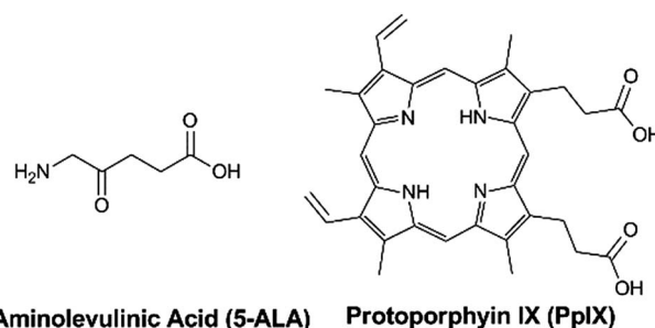
Fig. 1 Chemical structures.
