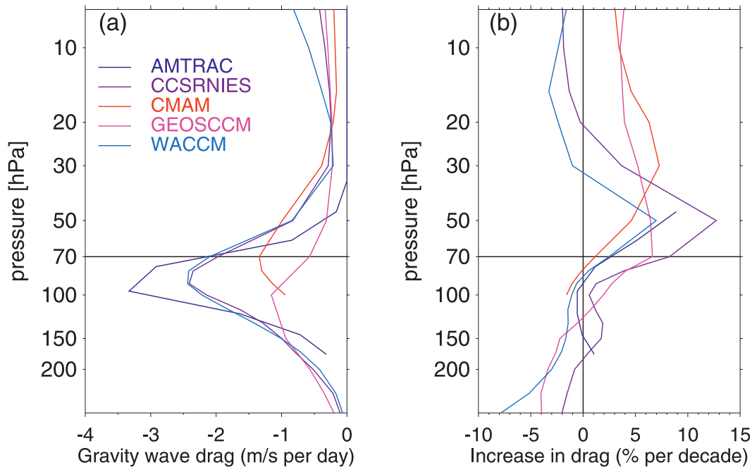
FIG. 12. (a) For the simulations of the AMTRAC, CCSRNIES model, CMAM, GEOS CCM, and WACCM, the vertical profiles of the annual mean orographic gravity wave drag [ \text{m s}^{-1} \text{ (day)}^{-1} ] at the latitudes north of the equator, where \bar{w}^* = 0 at 70 hPa. The annual mean is the average of the four seasonal means and therefore takes account of the seasonal cycle in the position where \bar{w}^* = 0 . The results shown are for the year 2000 based on a linear fit to the time series of annual mean vertical profiles. (b) Change in drag ( \% \text{ decade}^{-1} ) based on the linear fit to the time series. When results were available from more than one simulation of a particular model, the ensemble mean is shown. In the AMTRAC orographic gravity wave drag was set to zero above 42 hPa. The curves for the AMTRAC and the CMAM do not extend to the lowest levels because data were not provided for those levels. Nonetheless, it should be emphasized that the orographic GWD does operate throughout the depth of the troposphere in these models.
