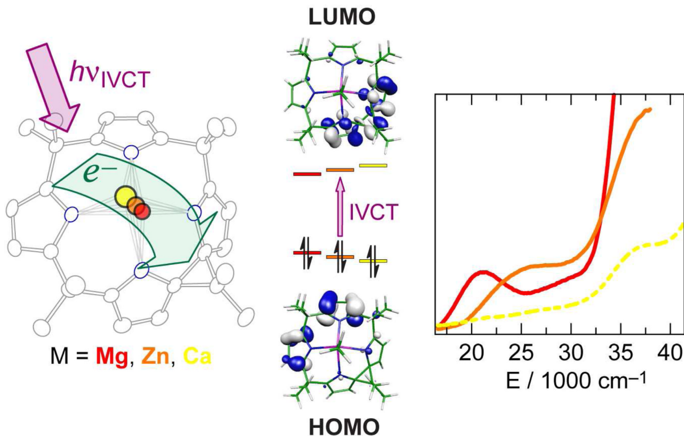
Figure 7. (Left) Thermal ellipsoid plot (50% probability level) for the solid-state structure of the two-electron mixed valence Mg porphyrinogen compound, [L^{\Delta}Mg(NCMe)] \cdot CH_2Cl_2 . (Middle) Computed frontier Kohn-Sham orbital diagram of the HOMO and LUMOs of [L^{\Delta}Mg(NCMe)] showing the localization of the electron density that gives rise to the ligand-to-ligand intravalence charge transfer transition (IVCT). (Right) UV-visible absorption spectra of [L^{\Delta}Mg] (—, red), [L^{\Delta}Zn] (---, orange) and [L^{\Delta}Ca] (---, yellow) in CH_2Cl_2 . Reproduced with permission from the Royal Society of Chemistry
