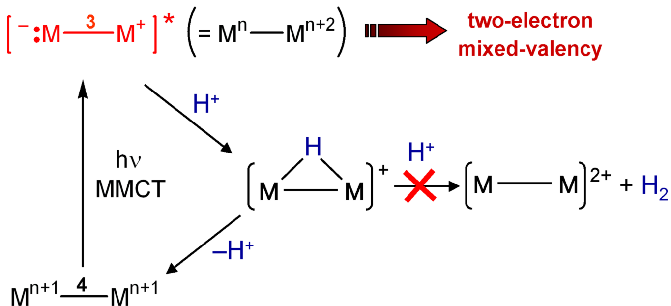
Figure 5. Metal-to-metal charge transfer (MMCT) produces a zwitterionic excited state in which the formal oxidation states of the metal differ by two. Transient absorption studies show that the excited state reacts with a proton to make a hydride, which back reacts to produce the \text{M}^{4-} -M grounds state. The hydride is not trapped by a second proton to produce hydrogen.
