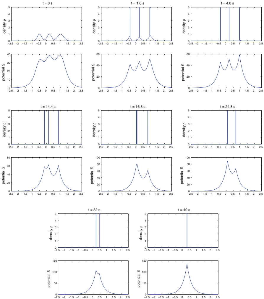
FIGURE 2. Dynamics of the density \rho (top) and of the potential S (bottom) for an initial density given by the sum of three Gaussian
