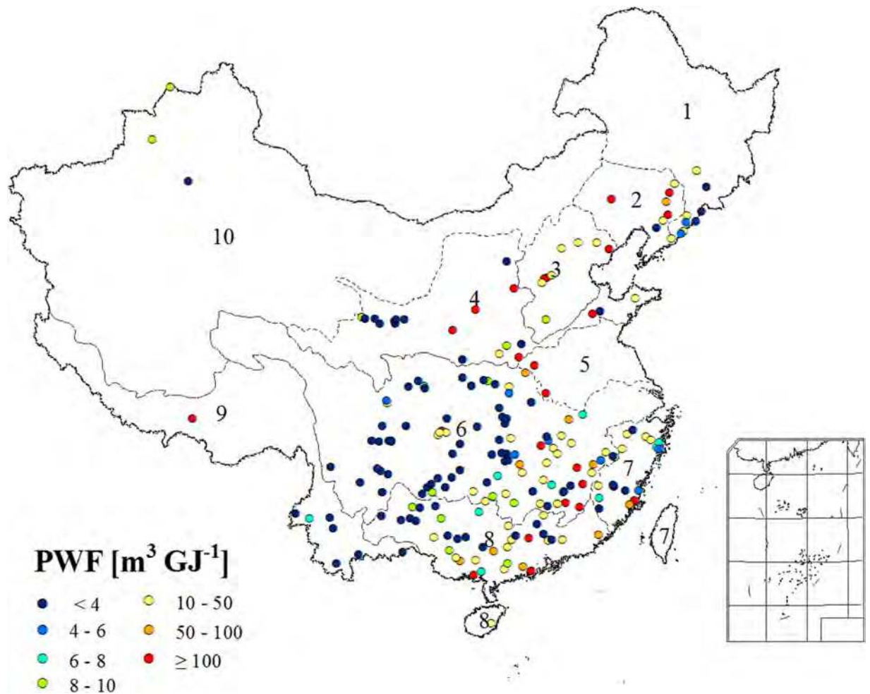
Figure 3. The product water footprint (PWF) of hydropower ( WF_h ) for 209 representative power plants in China. [Created with ArcGIS 9.3.1]
