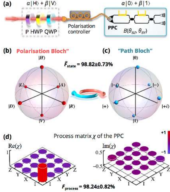
Fig. 2. Interconversion of polarization-encoding and path-encoding. (a) Initial arbitrary polarization-encoded states \alpha|H\rangle + \beta|V\rangle ( |H\rangle and |V\rangle are two orthogonal polarization states) were prepared by using a set of bulk optic polarizer (P), half-wave plate (HWP), and quarter-wave plate (QWP). A fiber-based polarization controller was used to compensate polarization rotation in the single mode fiber. The PPC interconverted the polarization-encoded states into on-chip path-encoded states \alpha|0\rangle + \beta|1\rangle , where |0\rangle and |1\rangle denote path states in two waveguides. The path-encoded states were then analyzed using the integrated analyzer B(\theta_{BZ}, \theta_{BY}) to implement state tomography. The Bloch sphere representation of, (b) ideal polarization-encoded states |H\rangle , |V\rangle , |D\rangle , |A\rangle , |L\rangle , and |R\rangle in bulk optics (red points), and (c) measured path-encoded states |0\rangle , |1\rangle , |+\rangle , |-\rangle , |+i\rangle , and | -i\rangle on chip (blue points). The density matrix presentation of all these states is provided in Supplement. Indicated fidelity represents the mean over the six measured states. (d) Reconstructed process matrix \chi of the PPC using the quantum process tomography.
